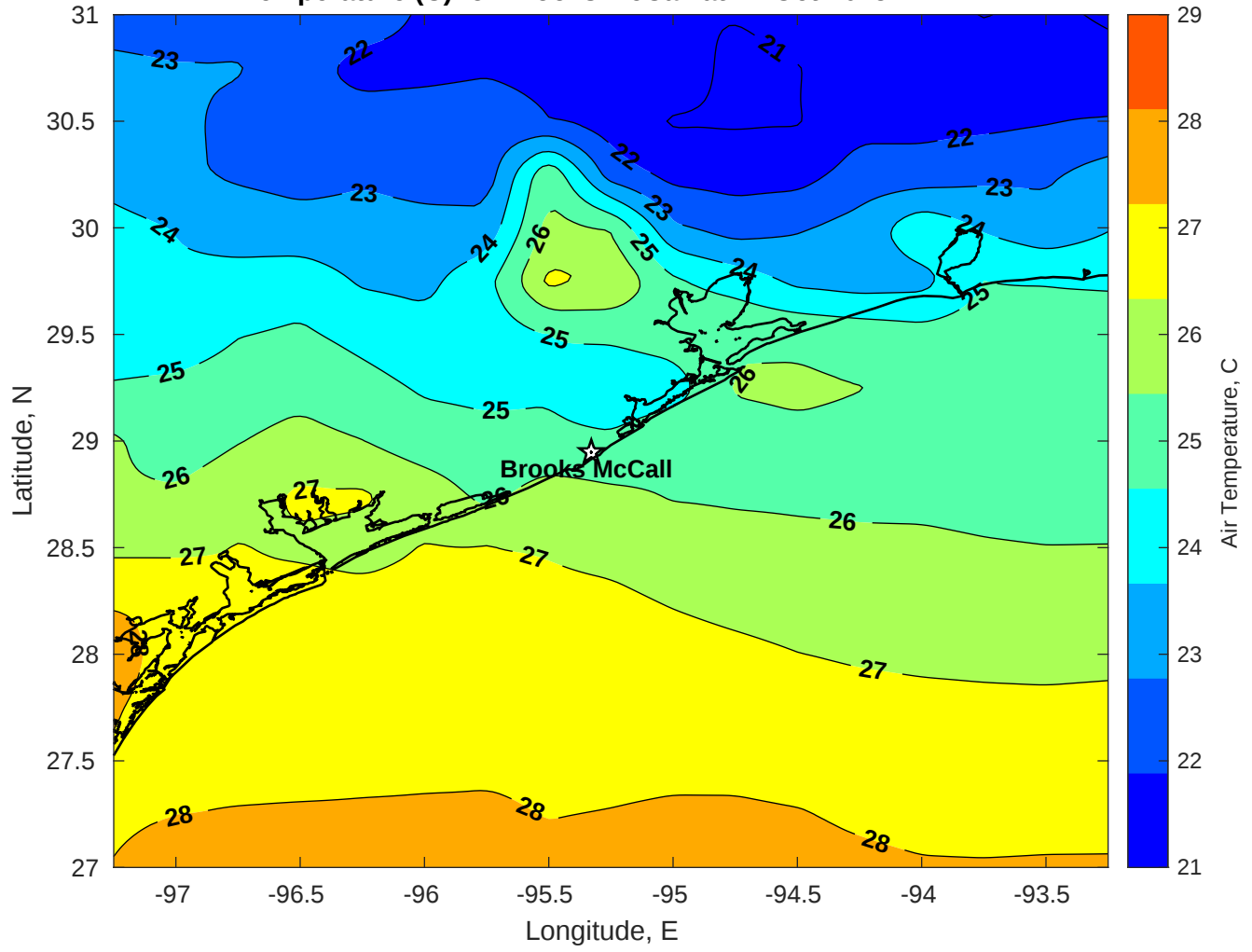
Air Temperature (C) for Brooks McCall at 27-Oct-2025
