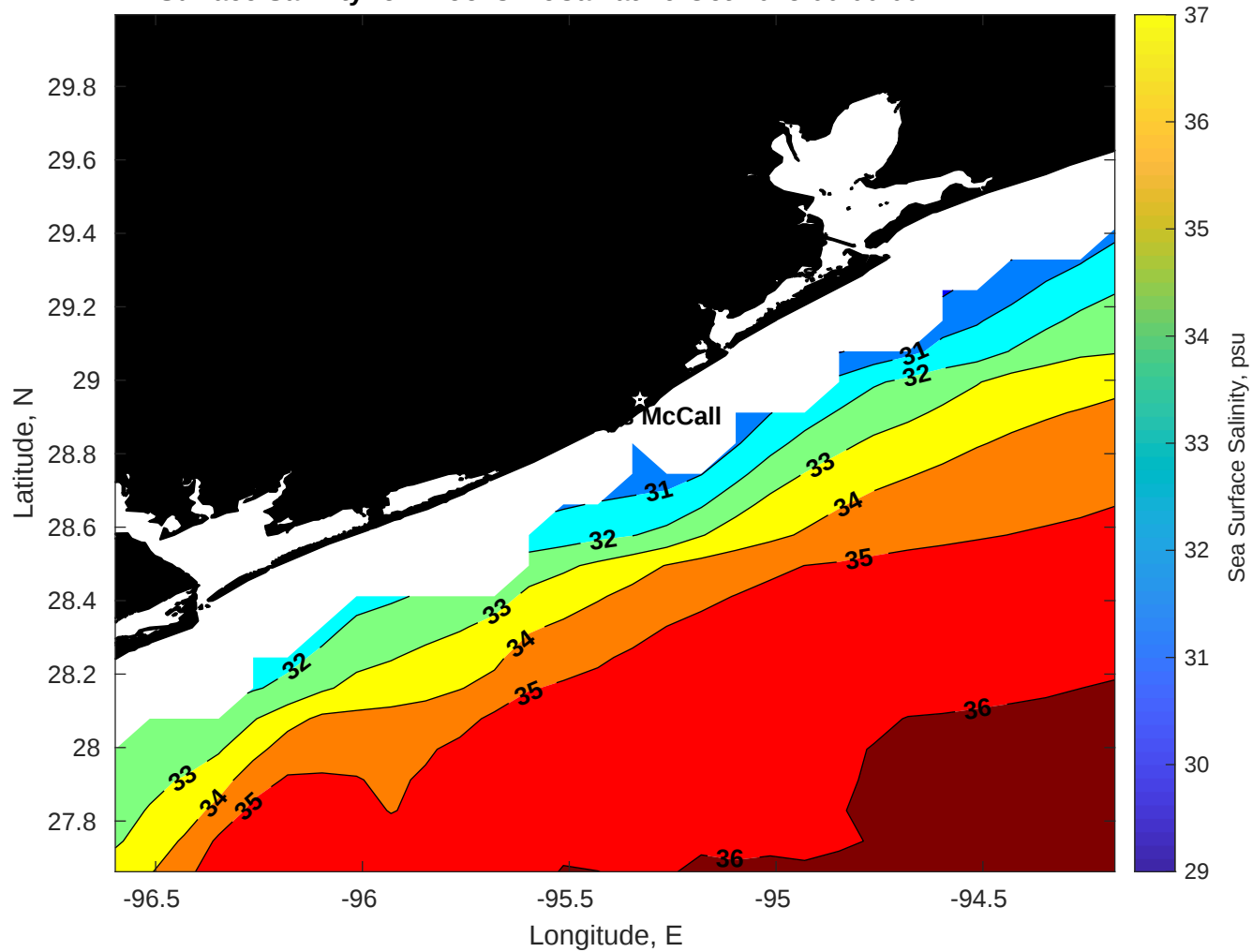
Surface Salinity for Brooks McCall at 26-Oct-2025 00:00:00
