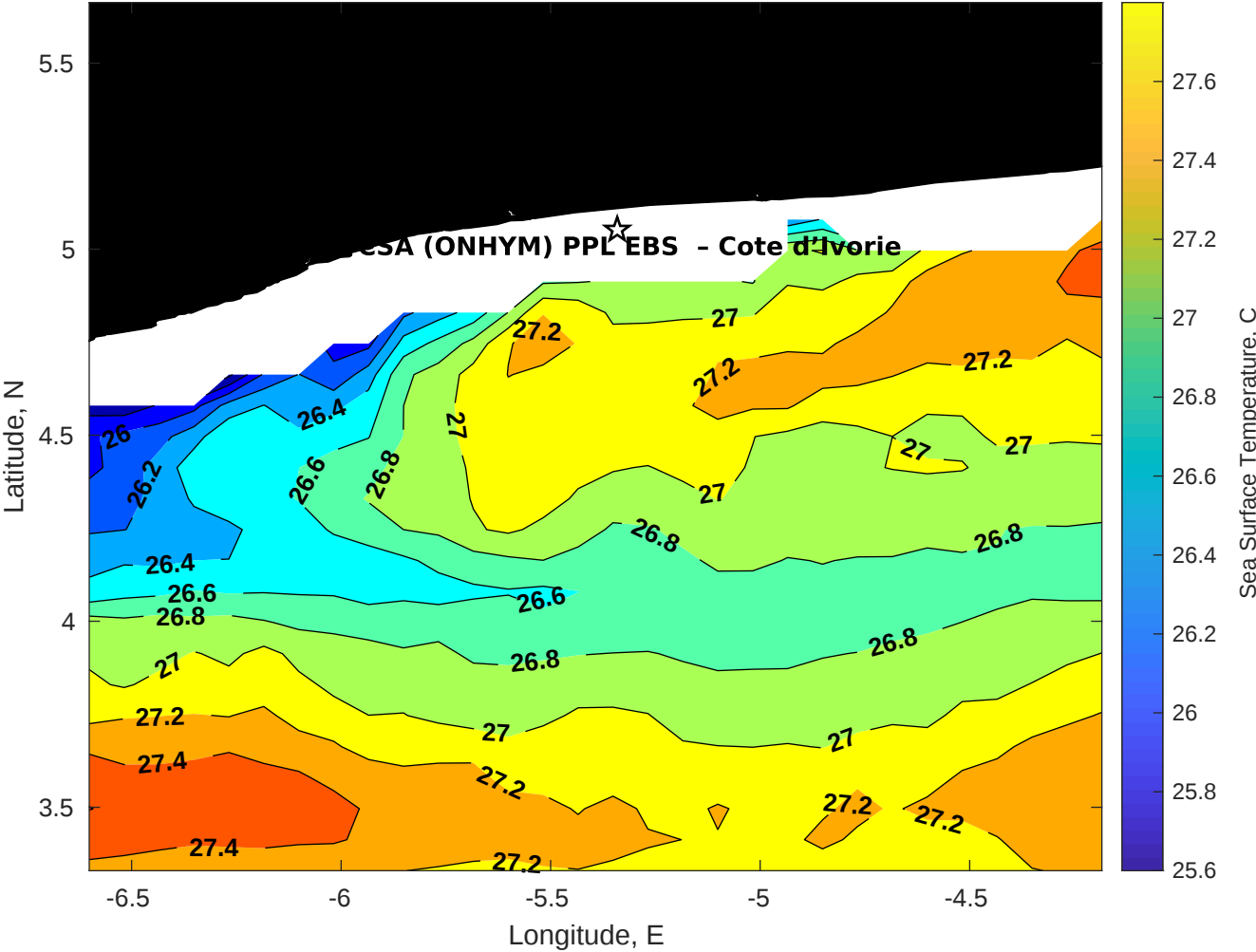
SST for CSA (ONHYM) PPL EBS - Cote d'Ivoire at 26-Oct-2025 00:00:00
