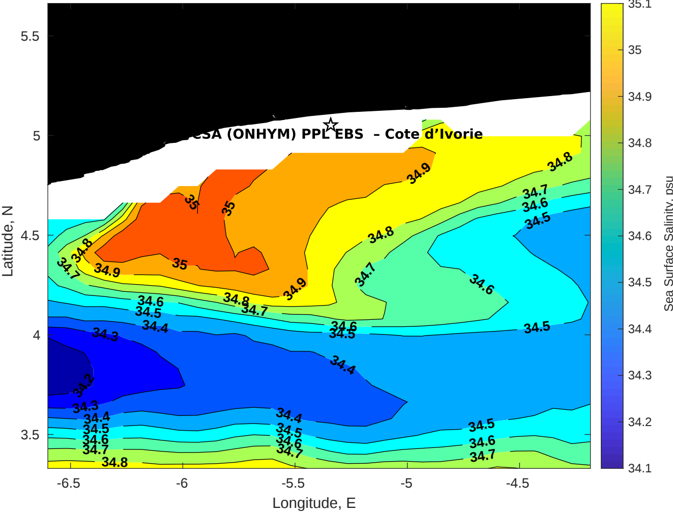
Surface Salinity for CSA (ONHYM) PPL EBS - Cote d'Ivoire at 26-Oct-2025 00:00:00
