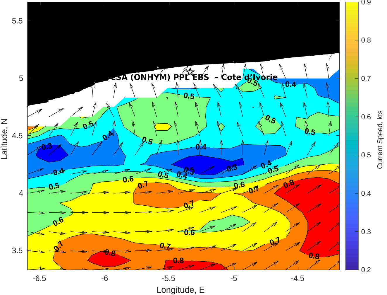
Surface Currents for CSA (ONHYM) PPL EBS - Cote d'Ivoire at 26-Oct-2025 00:00:00
