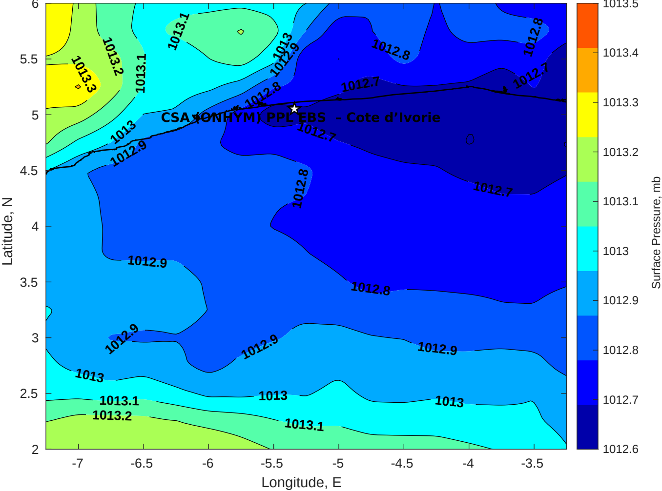
Surface Pressure (mb) for CSA (ONHYM) PPL EBS - Cote d'Ivoire at 27-Oct-2025 00:00:00
