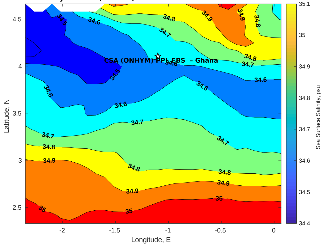
Surface Salinity for CSA (ONHYM) PPL EBS - Ghana at 26-Oct-2025 00:00:00
