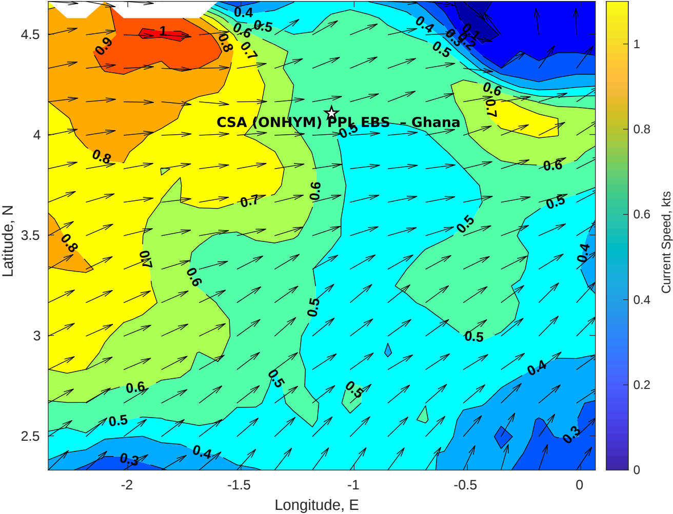
Surface Currents for CSA (ONHYM) PPL EBS - Ghana at 26-Oct-2025 00:00:00
