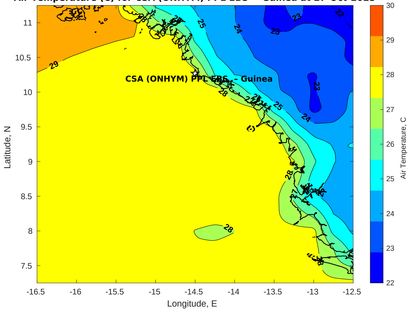
Air Temperature (C) for CSA (ONHYM) PPL EBS - Guinea at 27-Oct-2025
