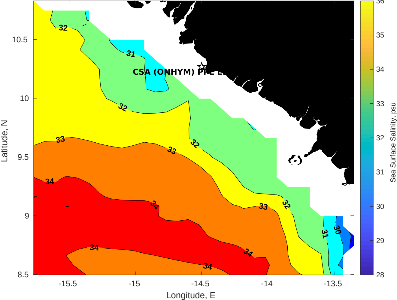
Surface Salinity for CSA (ONHYM) PPL EBS - Guinea at 26-Oct-2025 00:00:00
