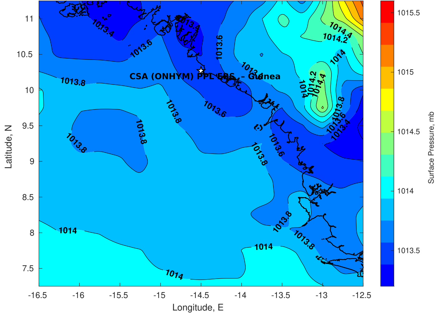
Surface Pressure (mb) for CSA (ONHYM) PPL EBS - Guinea at 29-Oct-2025 00:00:00
