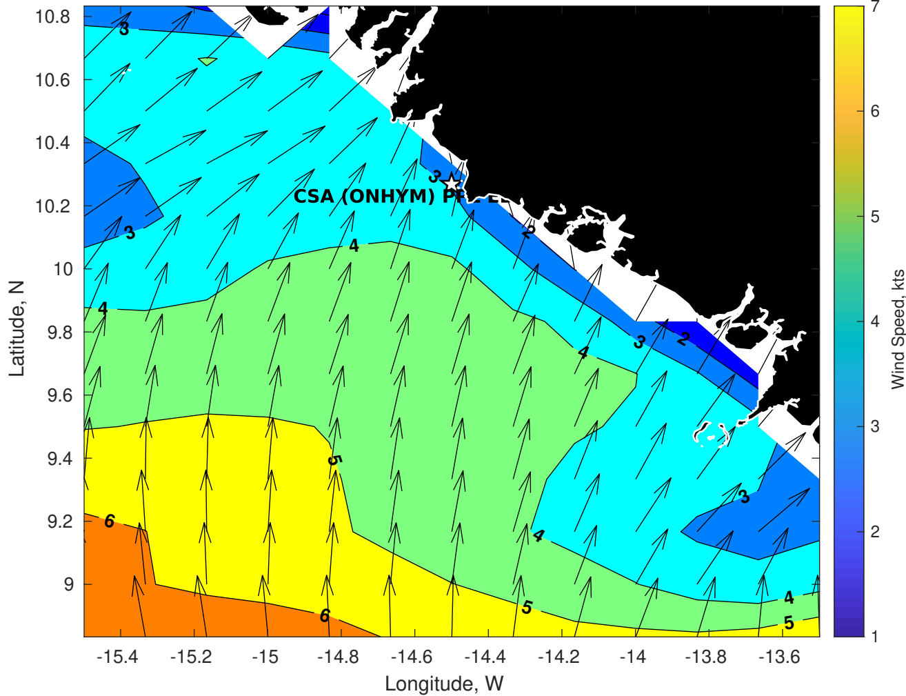
Winds (kts) for CSA (ONHYM) PPL EBS - Guinea at 27-Oct-2025 09:00:00
