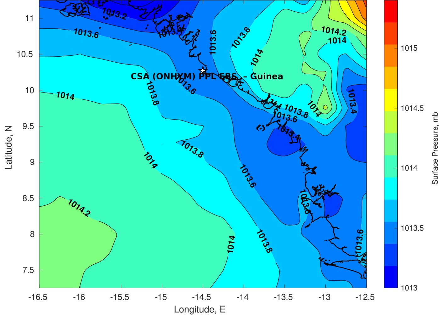
Surface Pressure (mb) for CSA (ONHYM) PPL EBS - Guinea at 28-Oct-2025 00:00:00
