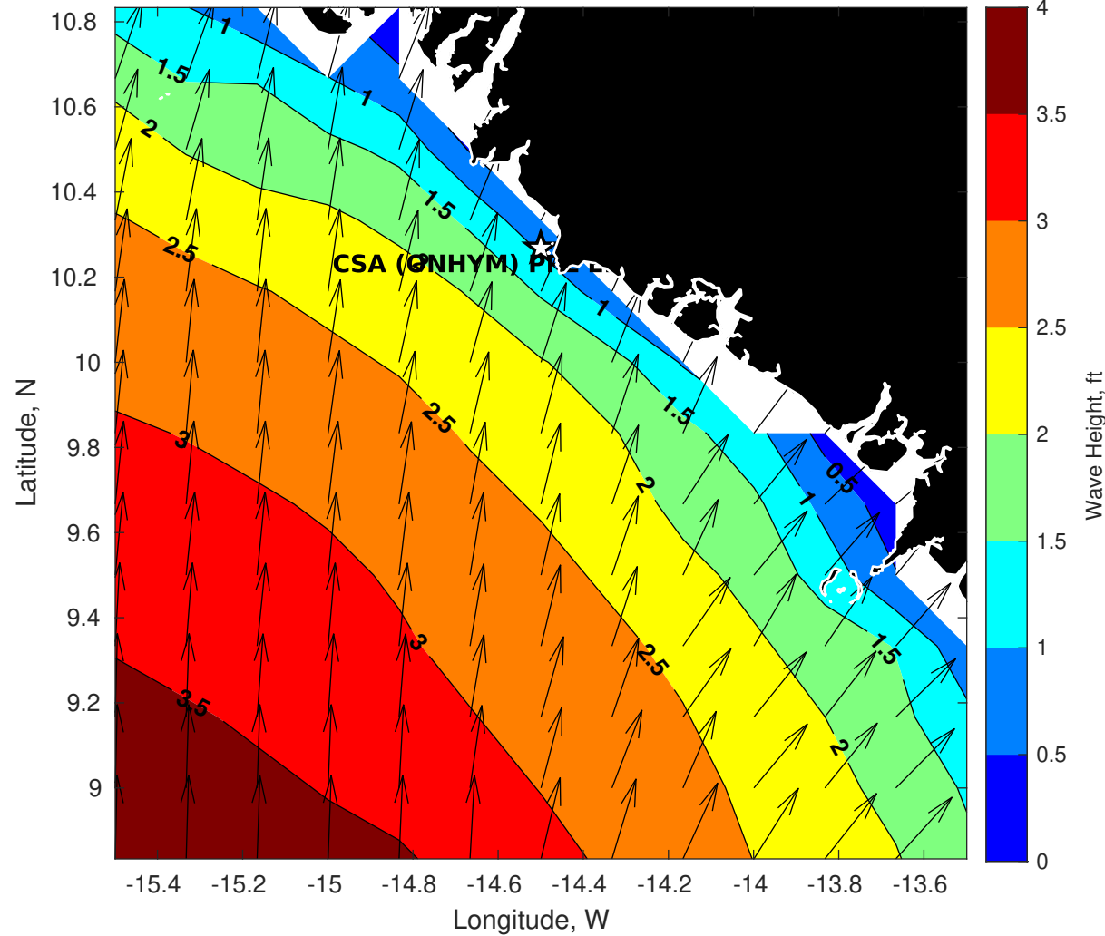
Wave Height (ft) for CSA (ONHYM) PPL EBS - Guinea at 27-Oct-2025 09:00:00
