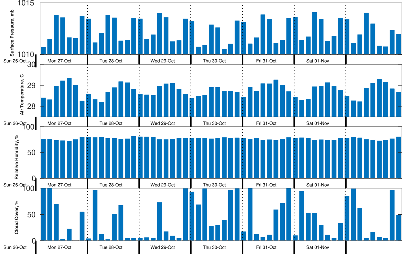
Met Forecast for CSA (ONHYM) PPL EBS - Guinea from 27-Oct-2025 00:00:00 to 03-Nov-2025 00:00:00
