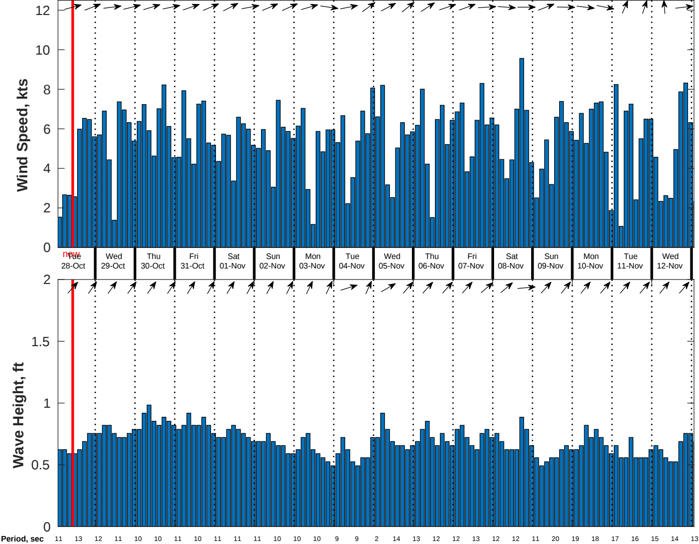
Wind & Wave Forecast for CSA (ONHYM) PPL EBS - Guinea from 27-Oct-2025 01:00:00 to 12-Nov-2025 01:00:00
