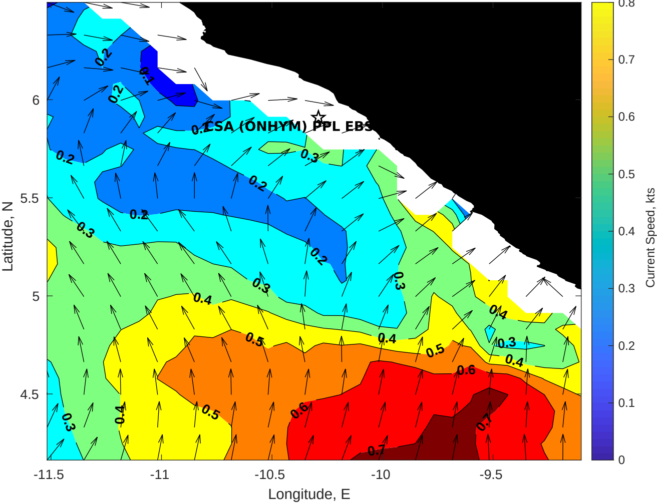
Surface Currents for CSA (ONHYM) PPL EBS - Liberia at 26-Oct-2025 00:00:00
