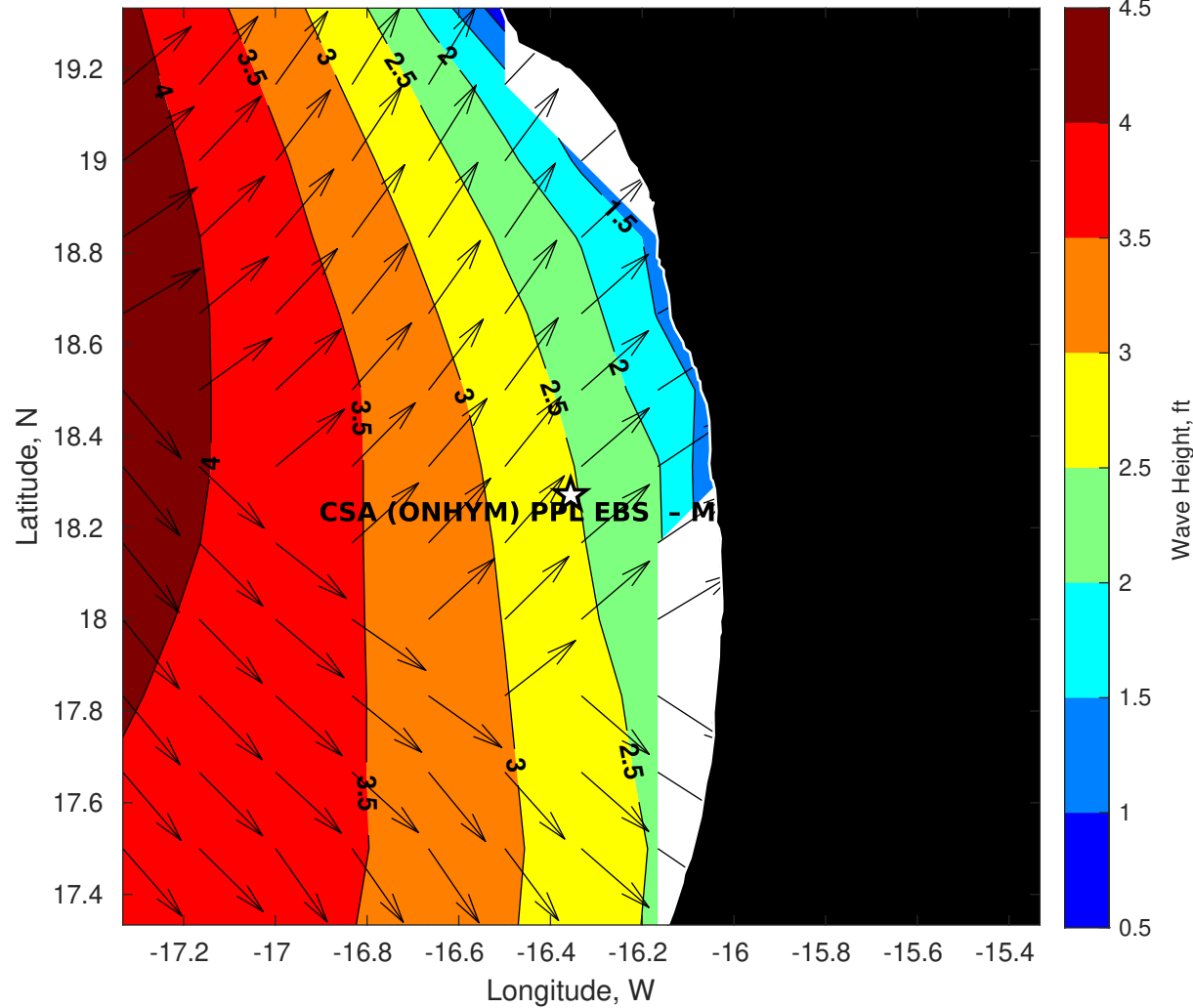
Wave Height (ft) for CSA (ONHYM) PPL EBS - Mauritania at 27-Oct-2025 09:00:00
