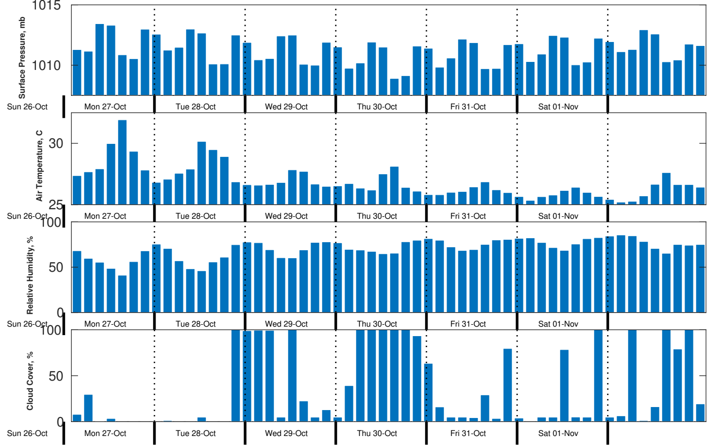
Met Forecast for CSA (ONHYM) PPL EBS - Mauritania from 27-Oct-2025 00:00:00 to 03-Nov-2025 00:00:00
