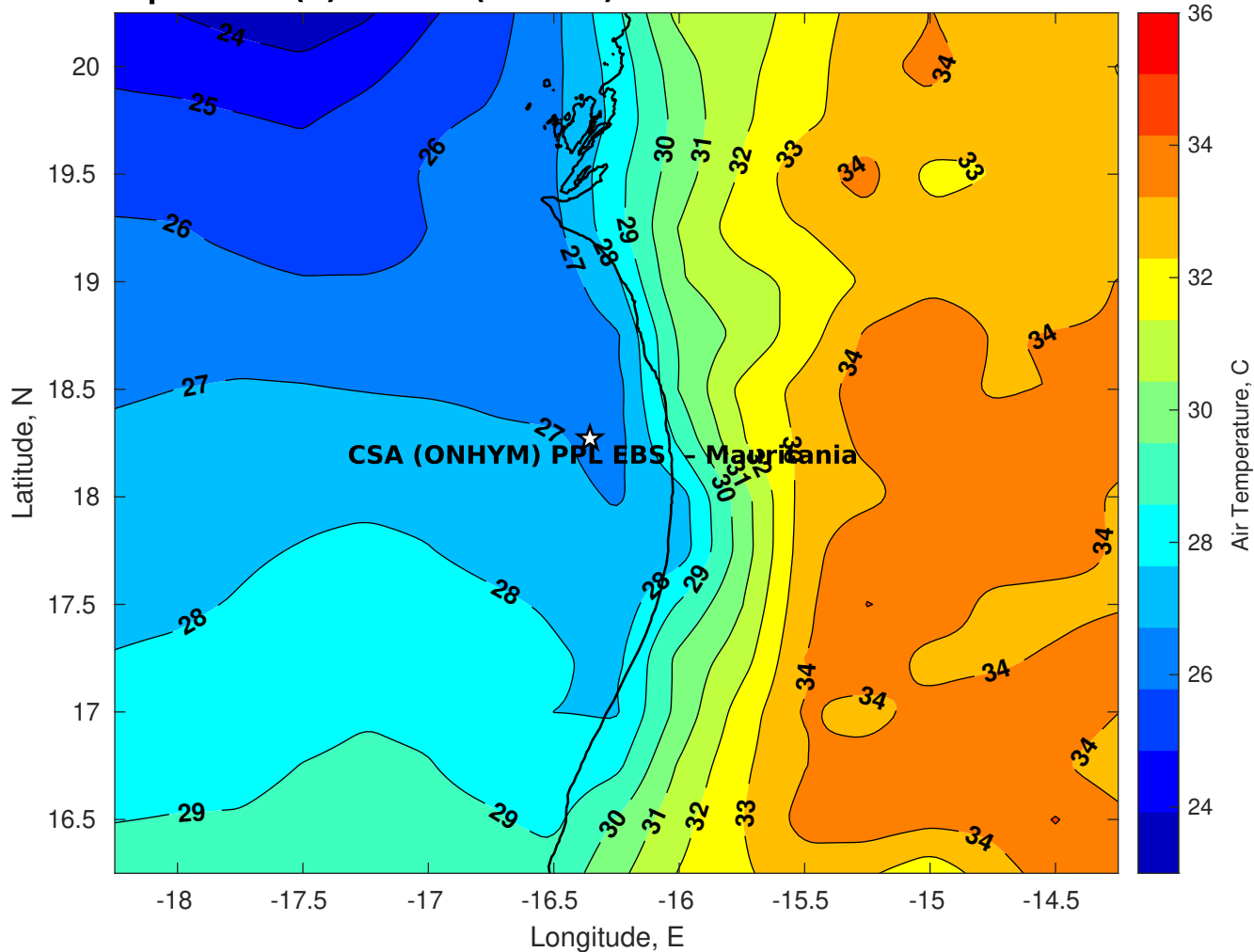
Air Temperature (C) for CSA (ONHYM) PPL EBS - Mauritania at 27-Oct-2025
