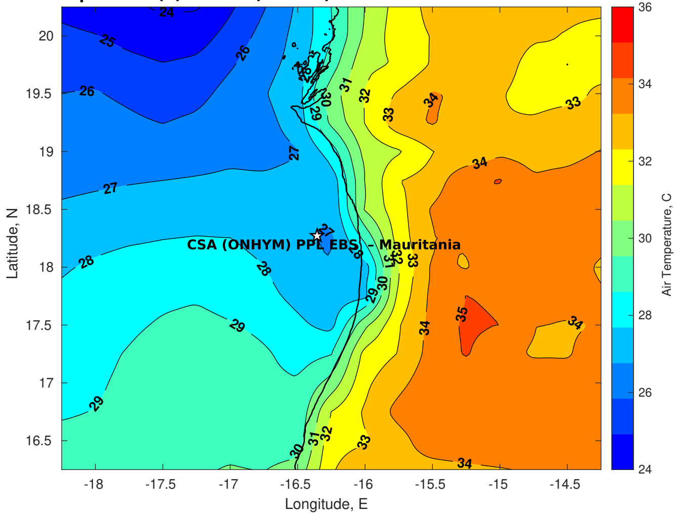
Air Temperature (C) for CSA (ONHYM) PPL EBS - Mauritania at 27-Oct-2025
