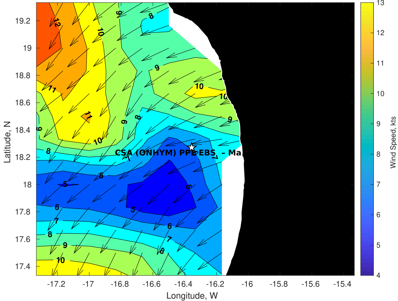
Winds (kts) for CSA (ONHYM) PPL EBS - Mauritania at 27-Oct-2025 09:00:00
