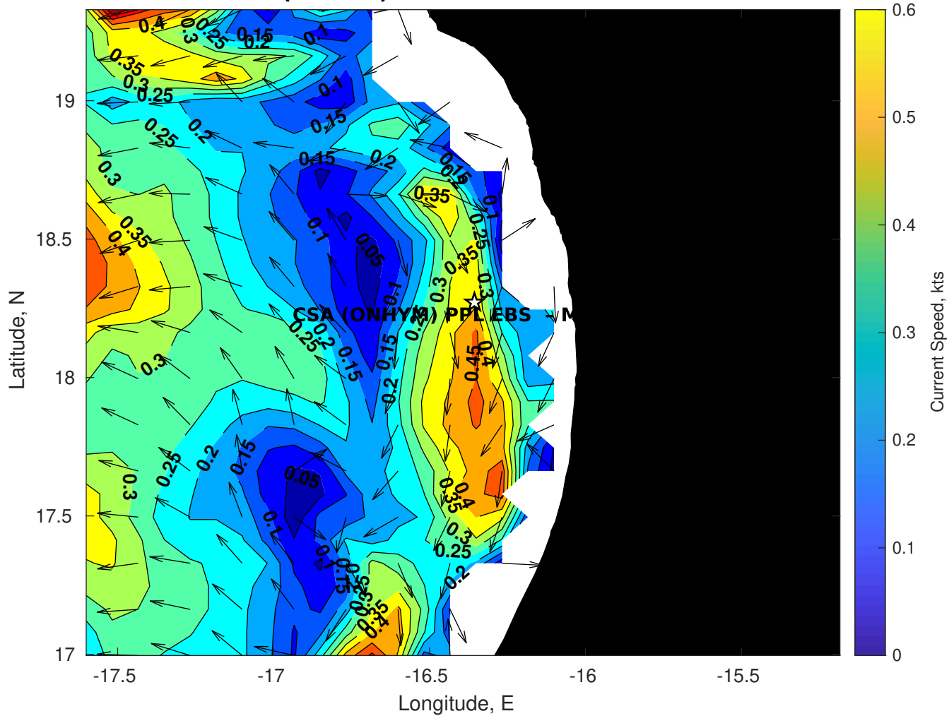
Surface Currents for CSA (ONHYM) PPL EBS - Mauritania at 26-Oct-2025 00:00:00
