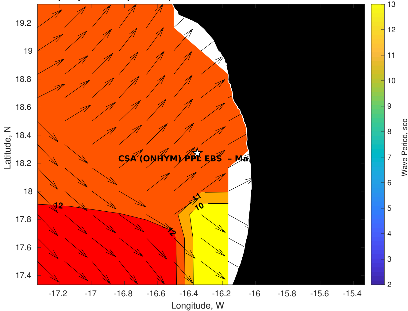
Wave Period (sec) for CSA (ONHYM) PPL EBS - Mauritania at 27-Oct-2025 09:00:00
