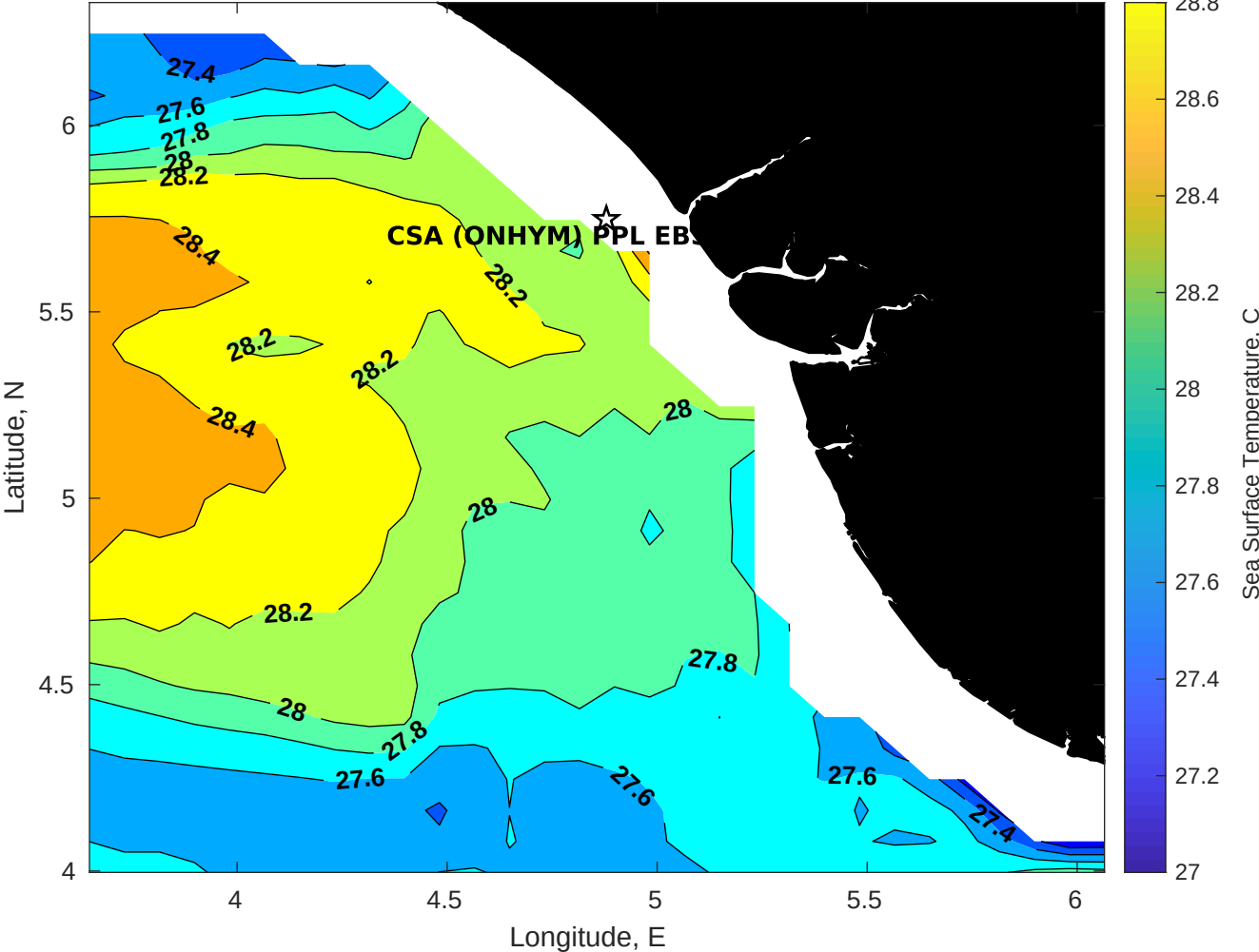
SST for CSA (ONHYM) PPL EBS - Nigeria at 26-Oct-2025 00:00:00
