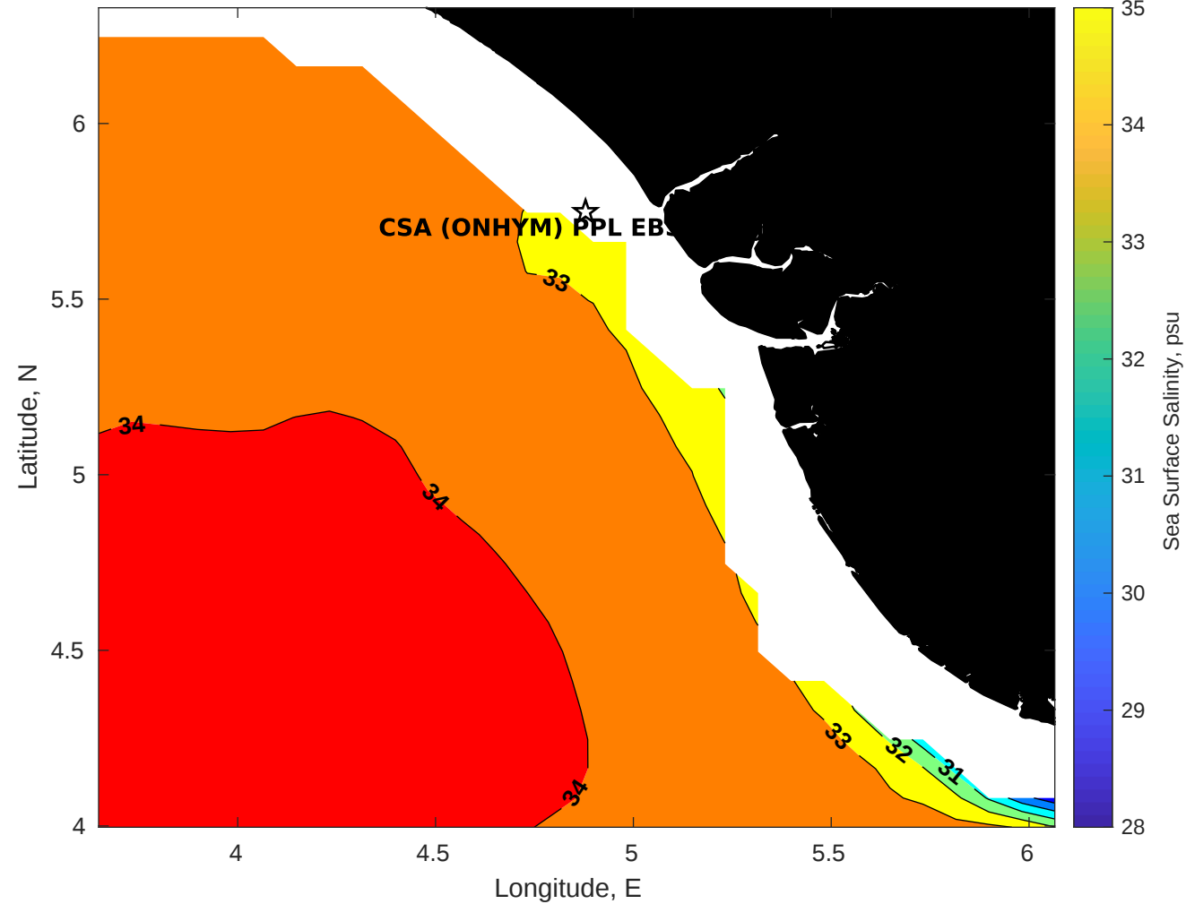
Surface Salinity for CSA (ONHYM) PPL EBS - Nigeria at 26-Oct-2025 00:00:00
