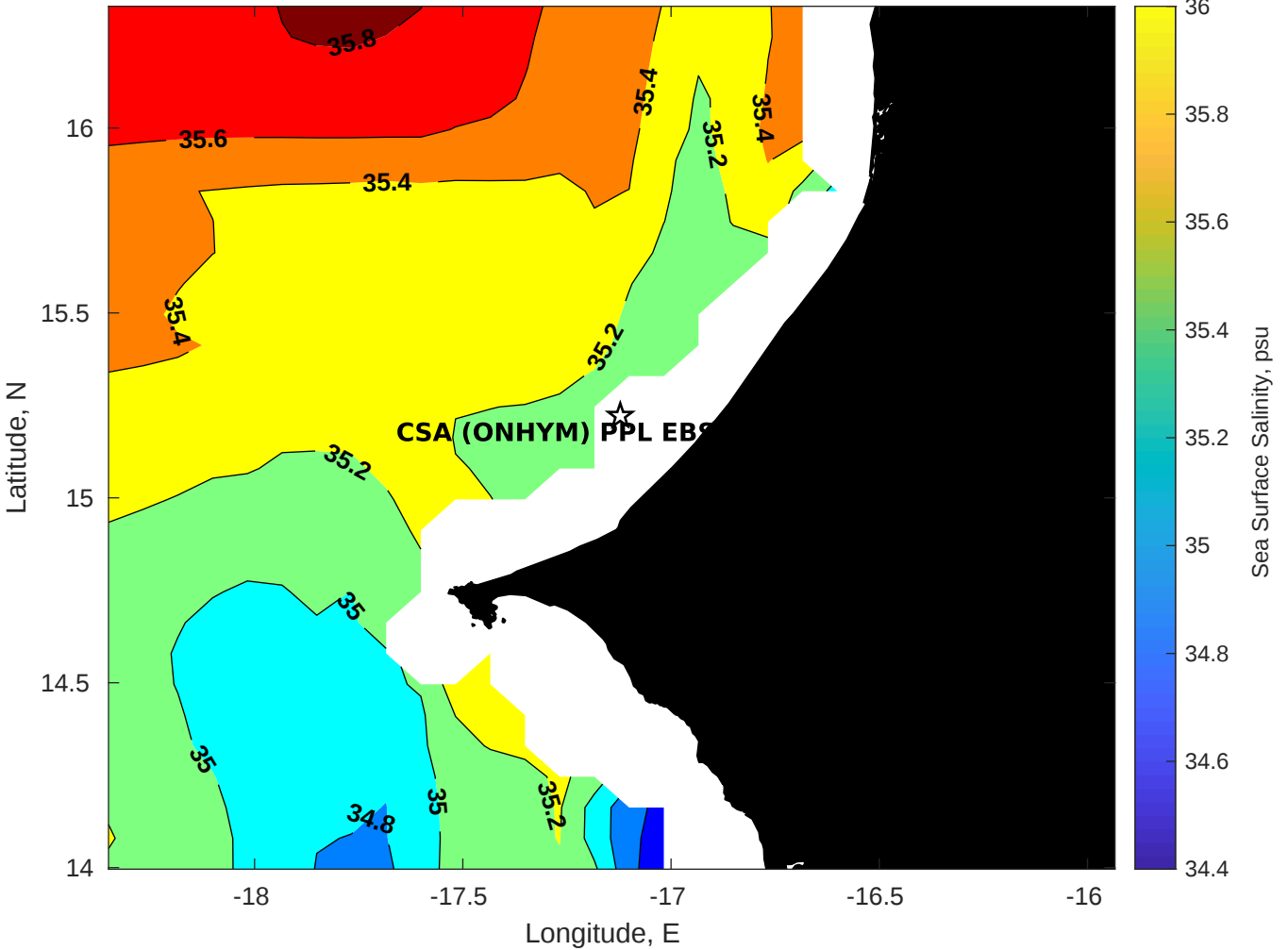
Surface Salinity for CSA (ONHYM) PPL EBS - Senegal at 26-Oct-2025 00:00:00
