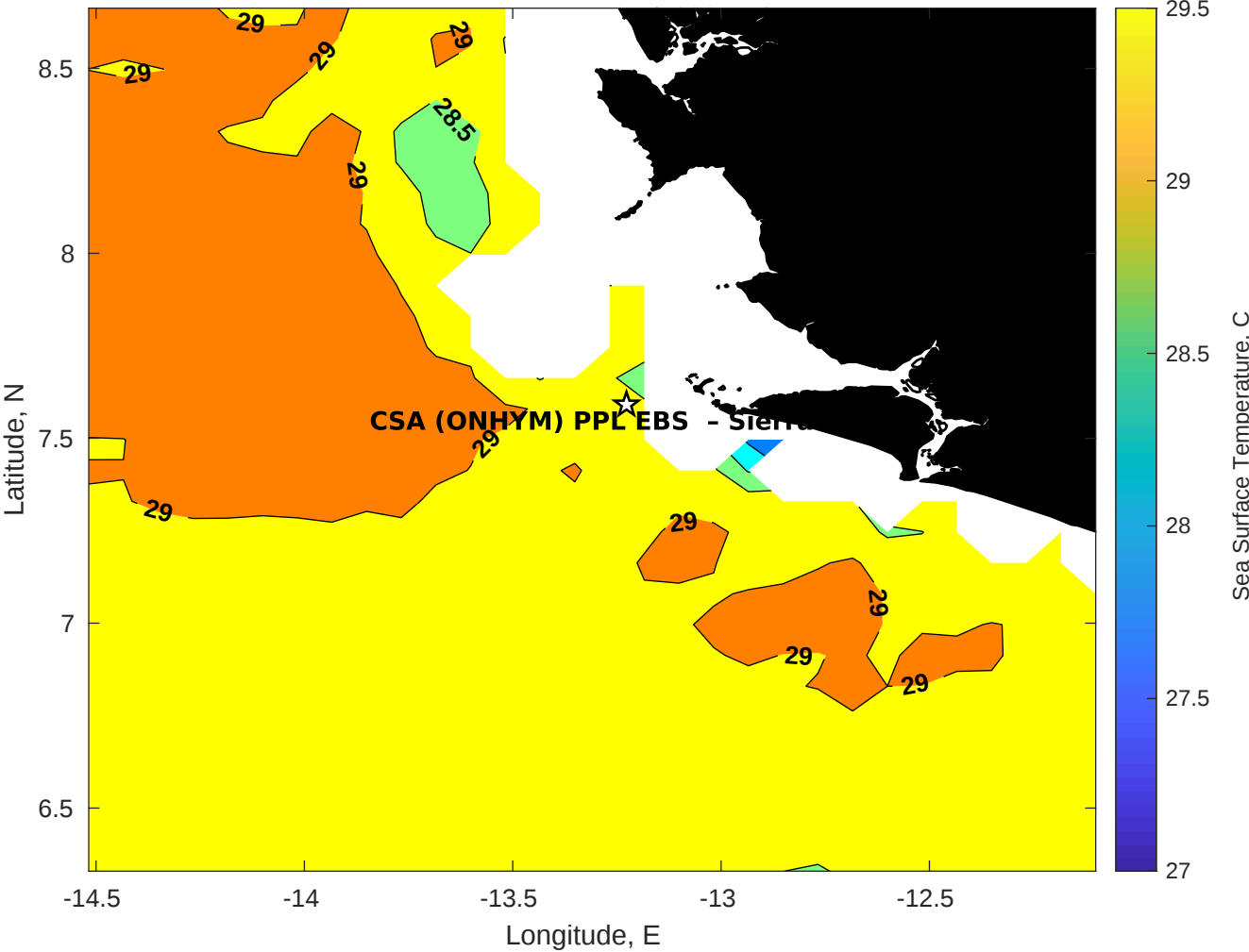
SST for CSA (ONHYM) PPL EBS - Sierra Leone at 26-Oct-2025 00:00:00
