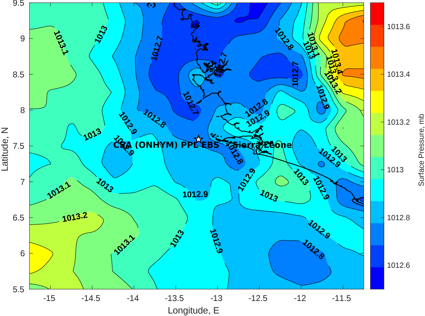
Surface Pressure (mb) for CSA (ONHYM) PPL EBS - Sierra Leone at 27-Oct-2025 00:00:00
