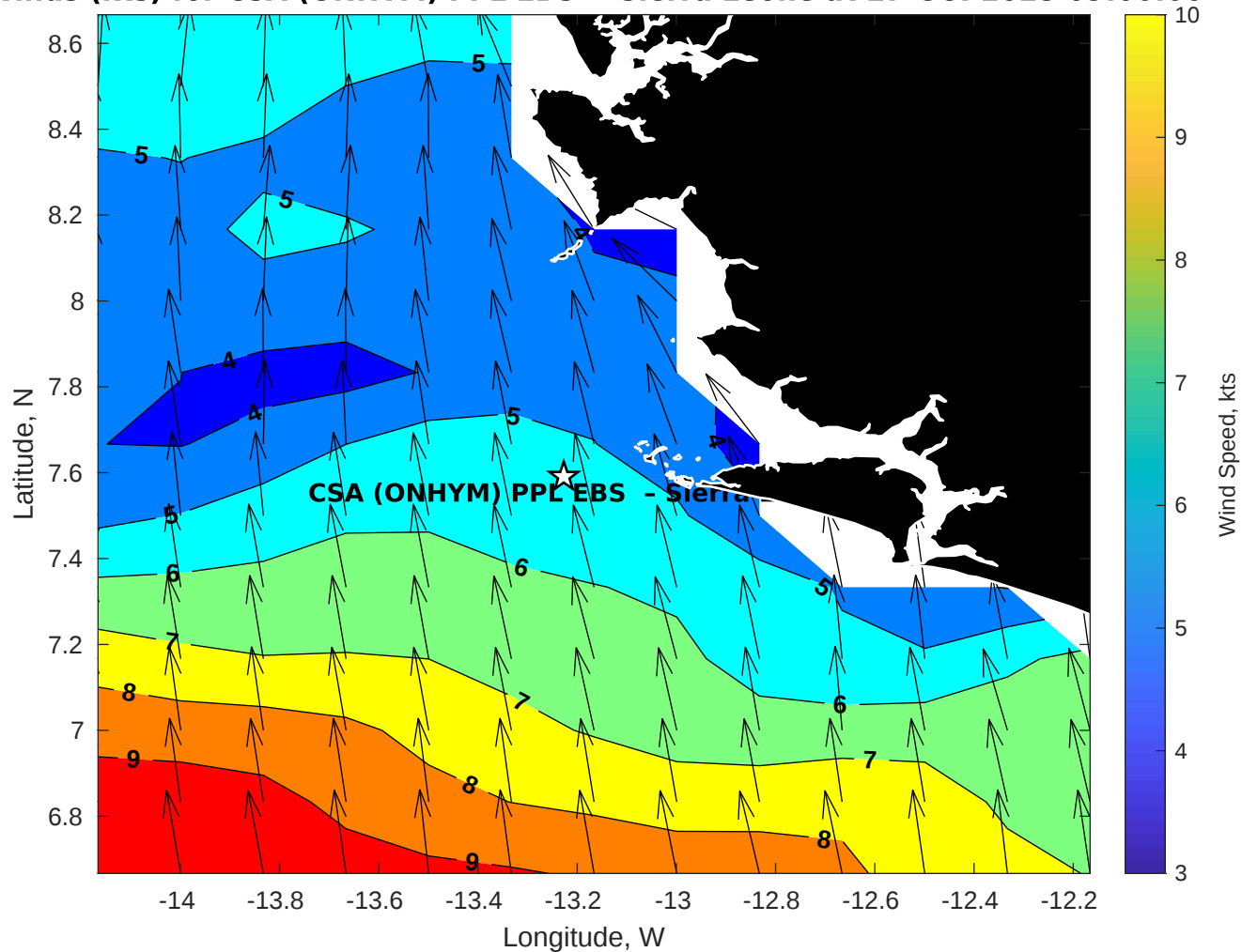
Winds (kts) for CSA (ONHYM) PPL EBS - Sierra Leone at 27-Oct-2025 09:00:00
