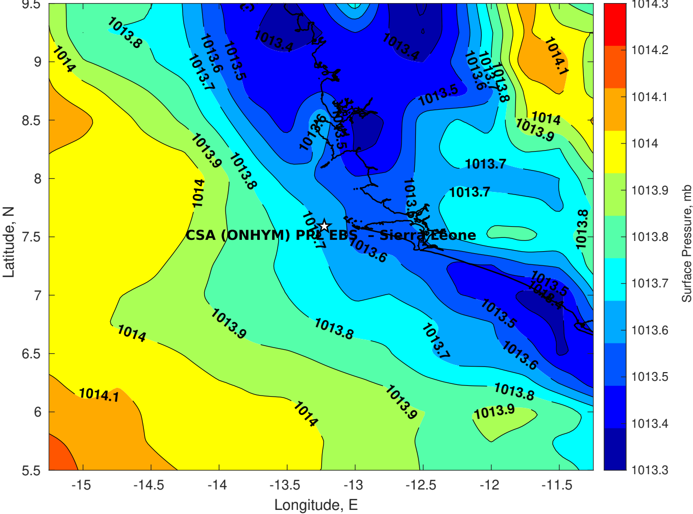
Surface Pressure (mb) for CSA (ONHYM) PPL EBS - Sierra Leone at 28-Oct-2025 00:00:00
