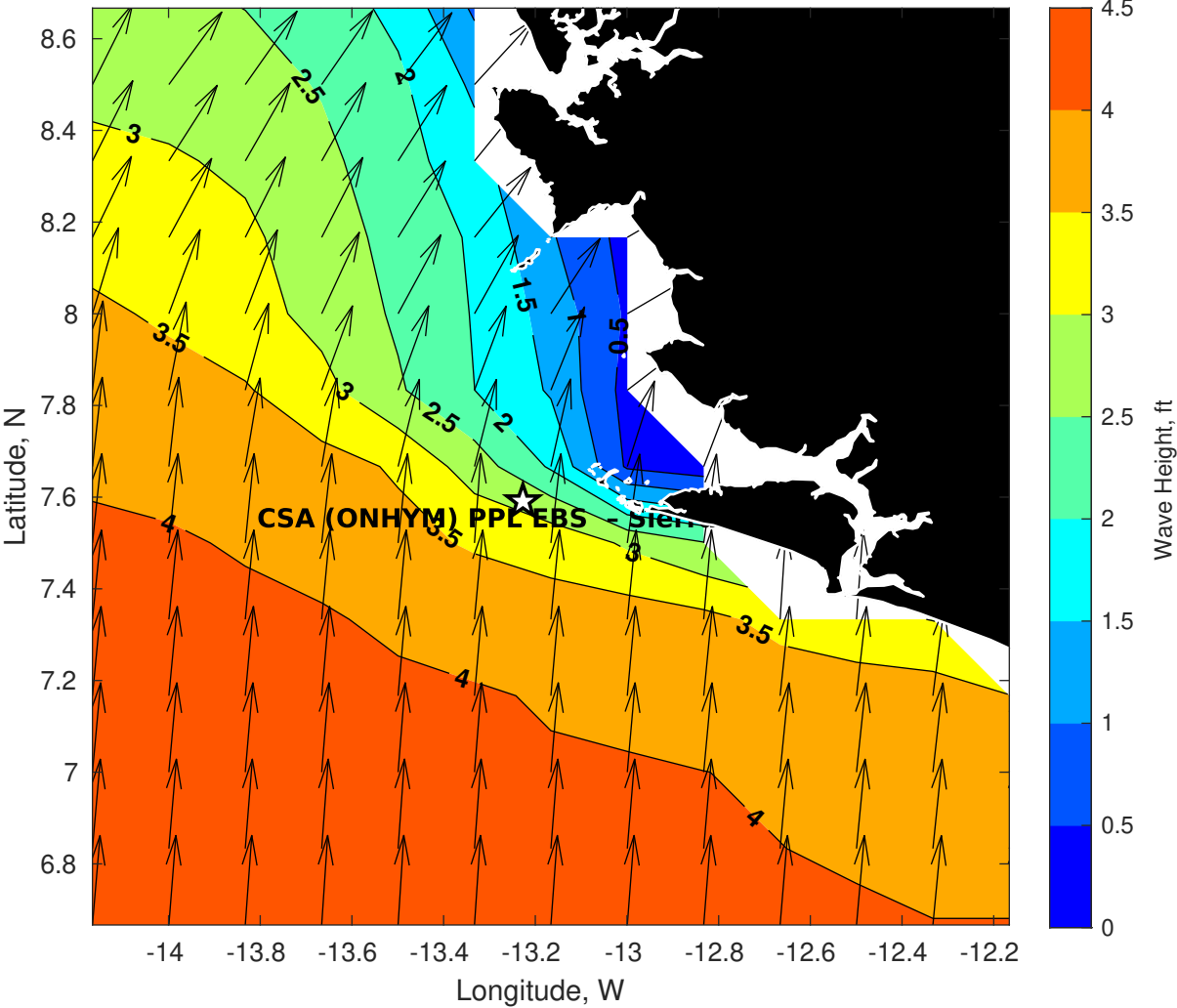
Wave Height (ft) for CSA (ONHYM) PPL EBS - Sierra Leone at 27-Oct-2025 09:00:00
