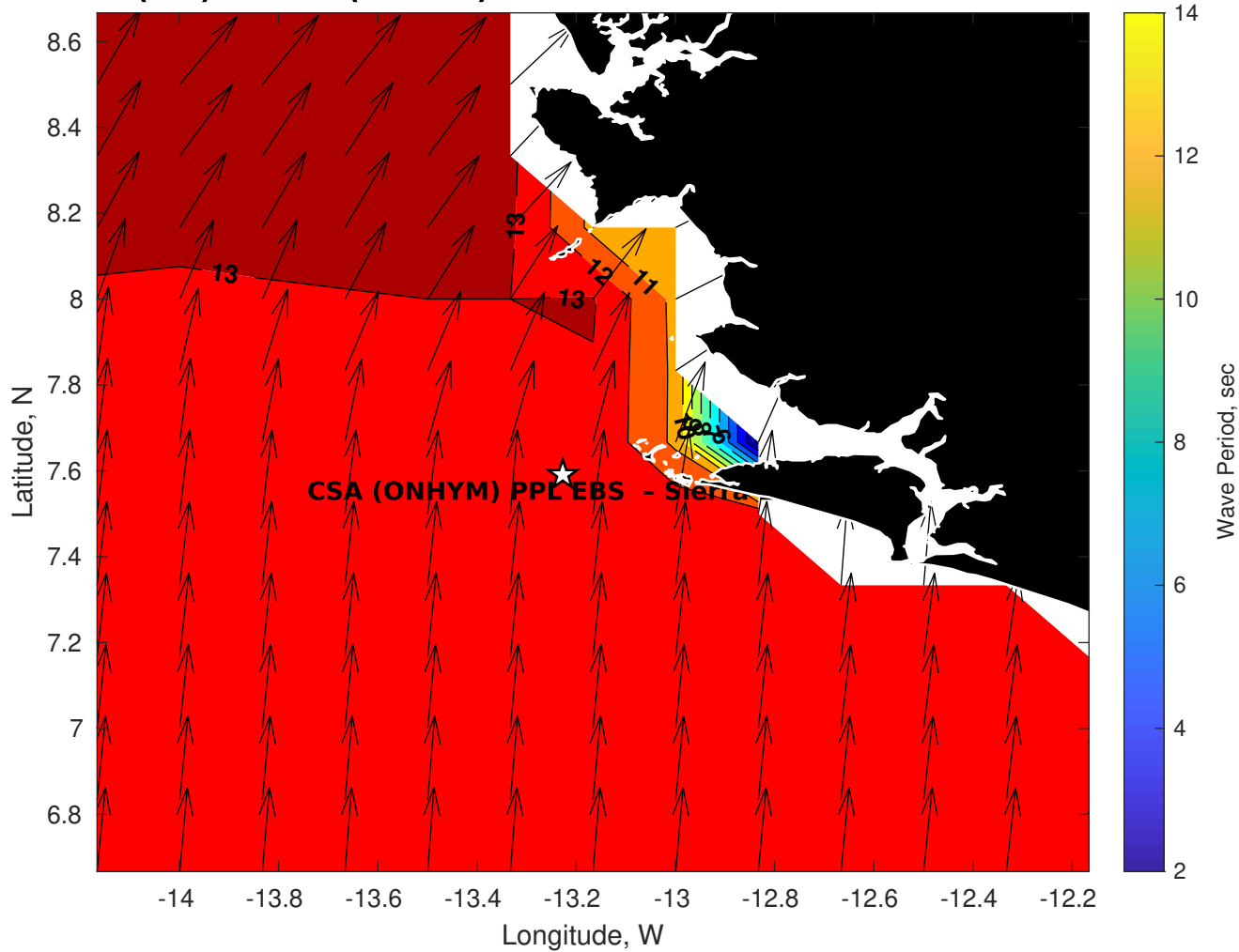
Wave Period (sec) for CSA (ONHYM) PPL EBS - Sierra Leone at 27-Oct-2025 09:00:00
