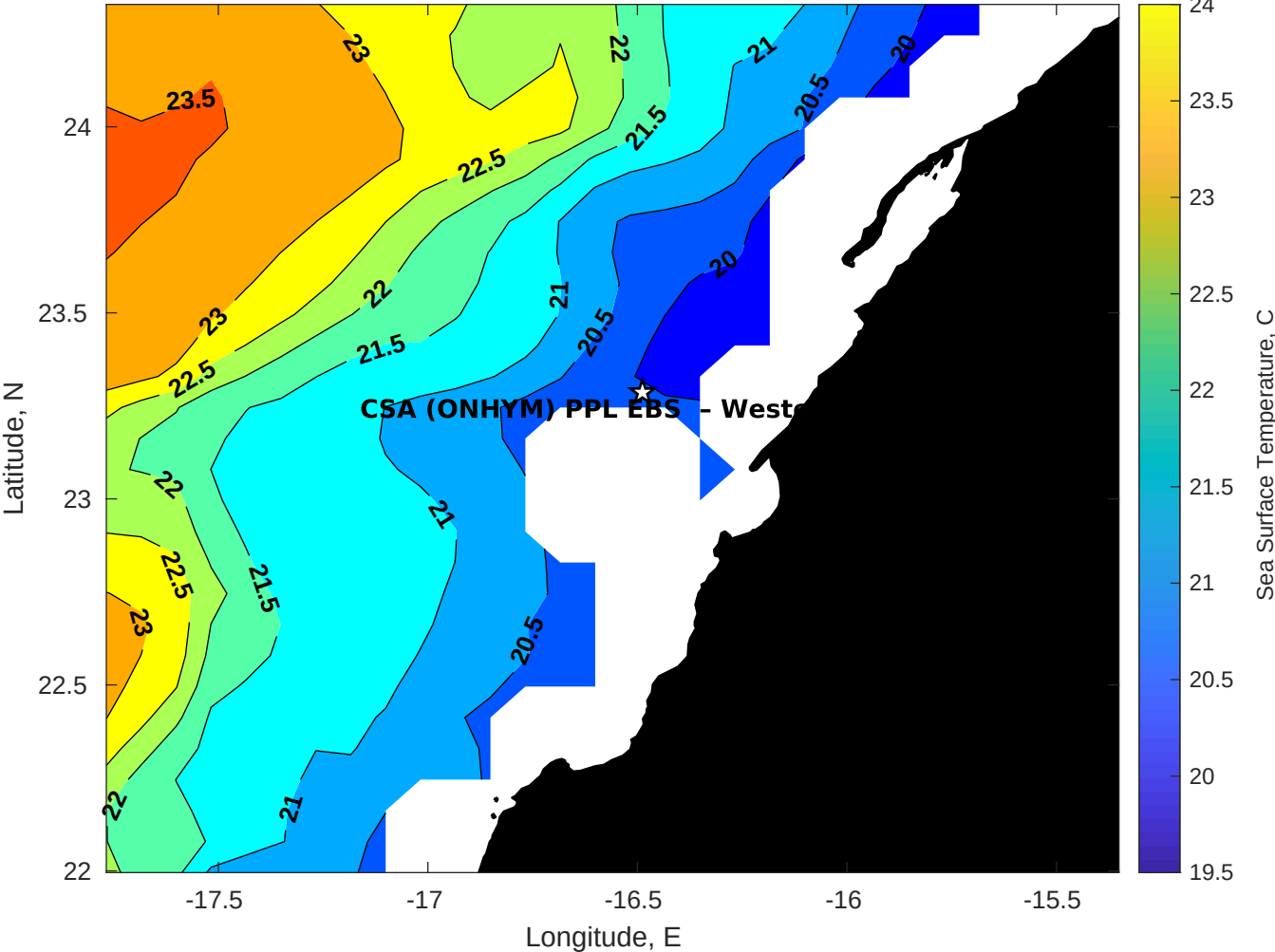
SST for CSA (ONHYM) PPL EBS - Western Sahara at 26-Oct-2025 00:00:00
