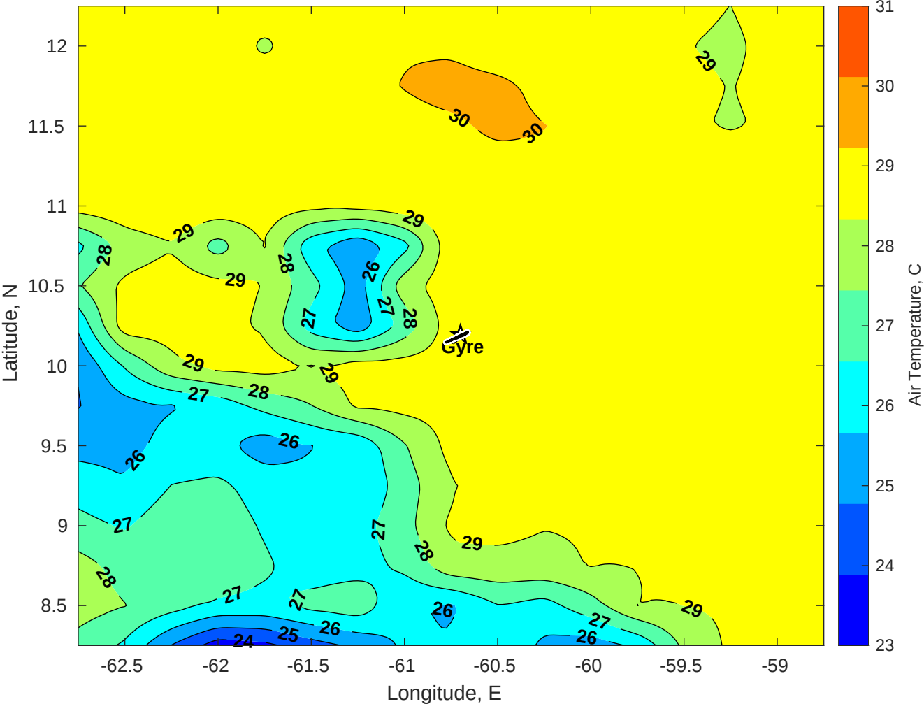
Air Temperature (C) for Gyre at 27-Oct-2025
