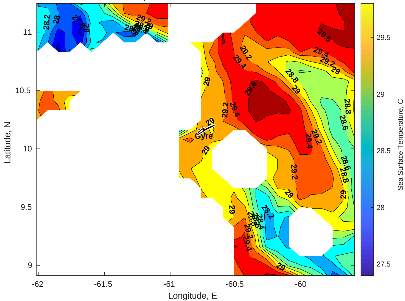
SST for Gyre at 26-Oct-2025 00:00:00
