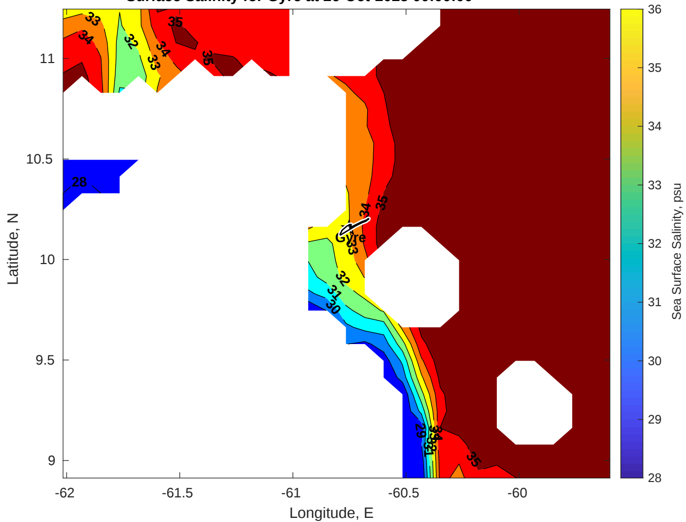
Surface Salinity for Gyre at 26-Oct-2025 00:00:00
