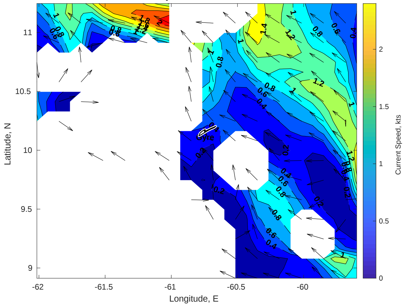
Surface Currents for Gyre at 26-Oct-2025 00:00:00
