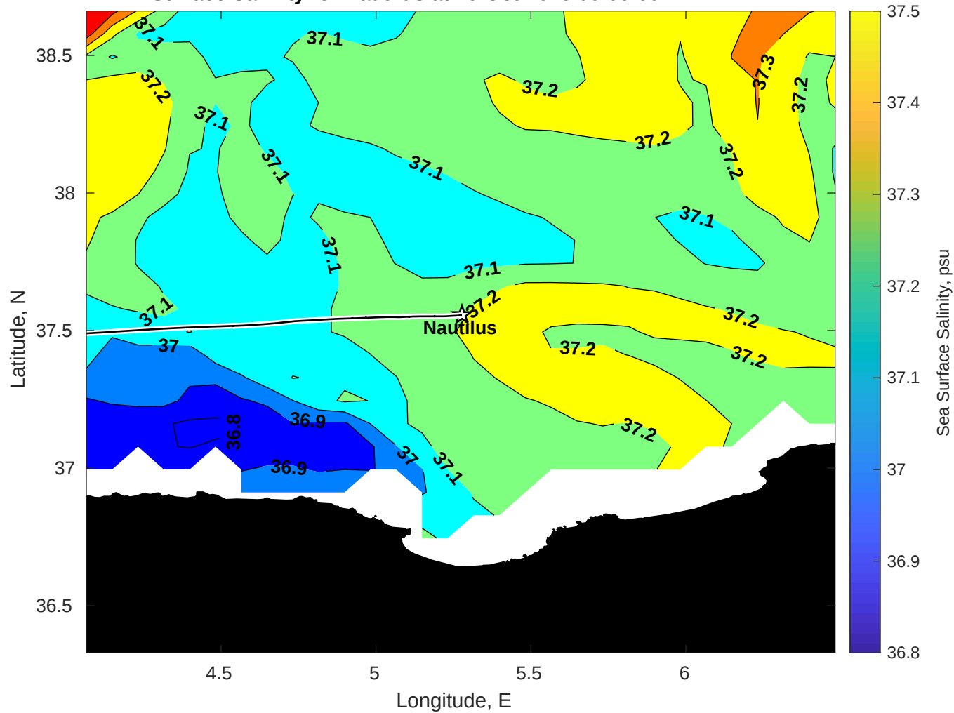
Surface Salinity for Nautilus at 26-Oct-2025 00:00:00
