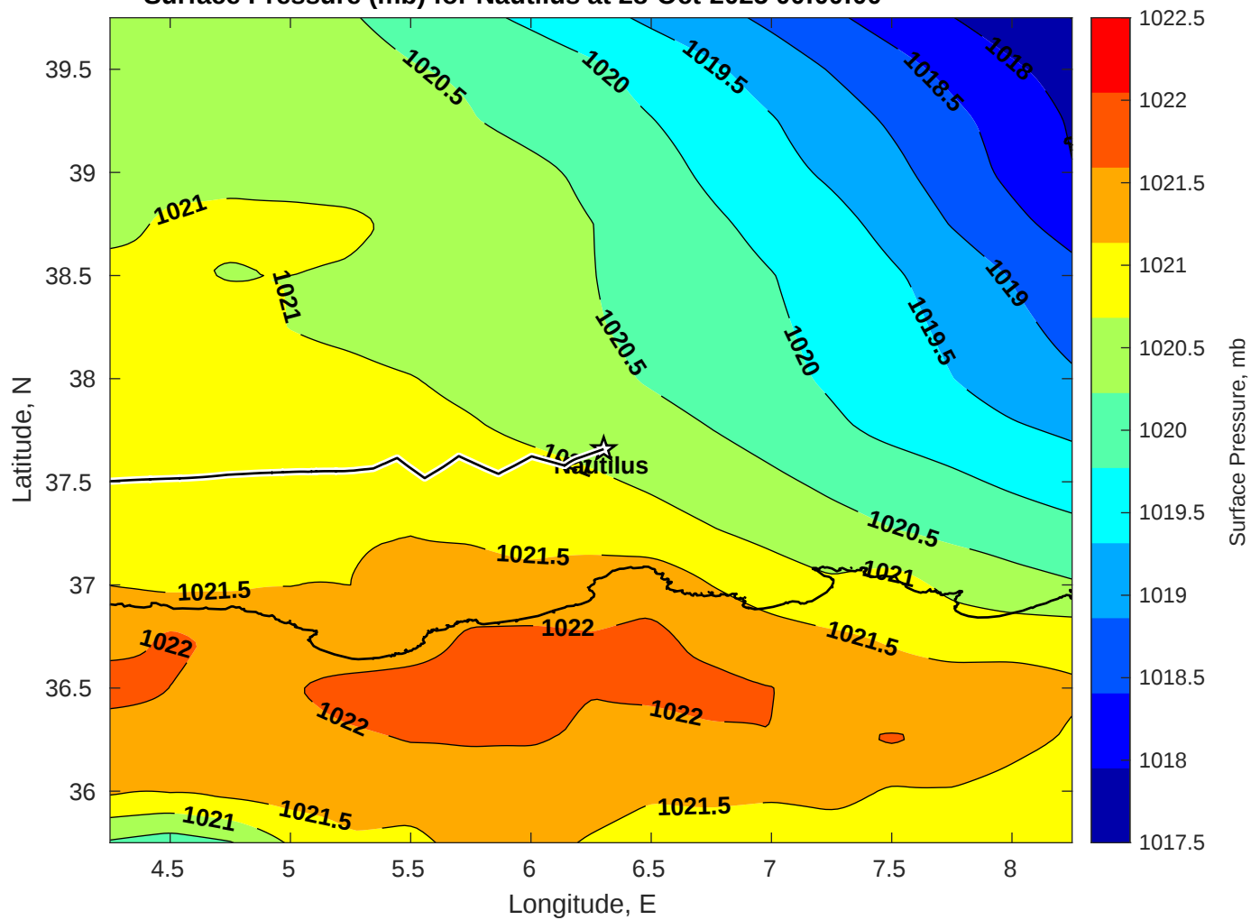
Surface Pressure (mb) for Nautilus at 28-Oct-2025 00:00:00
