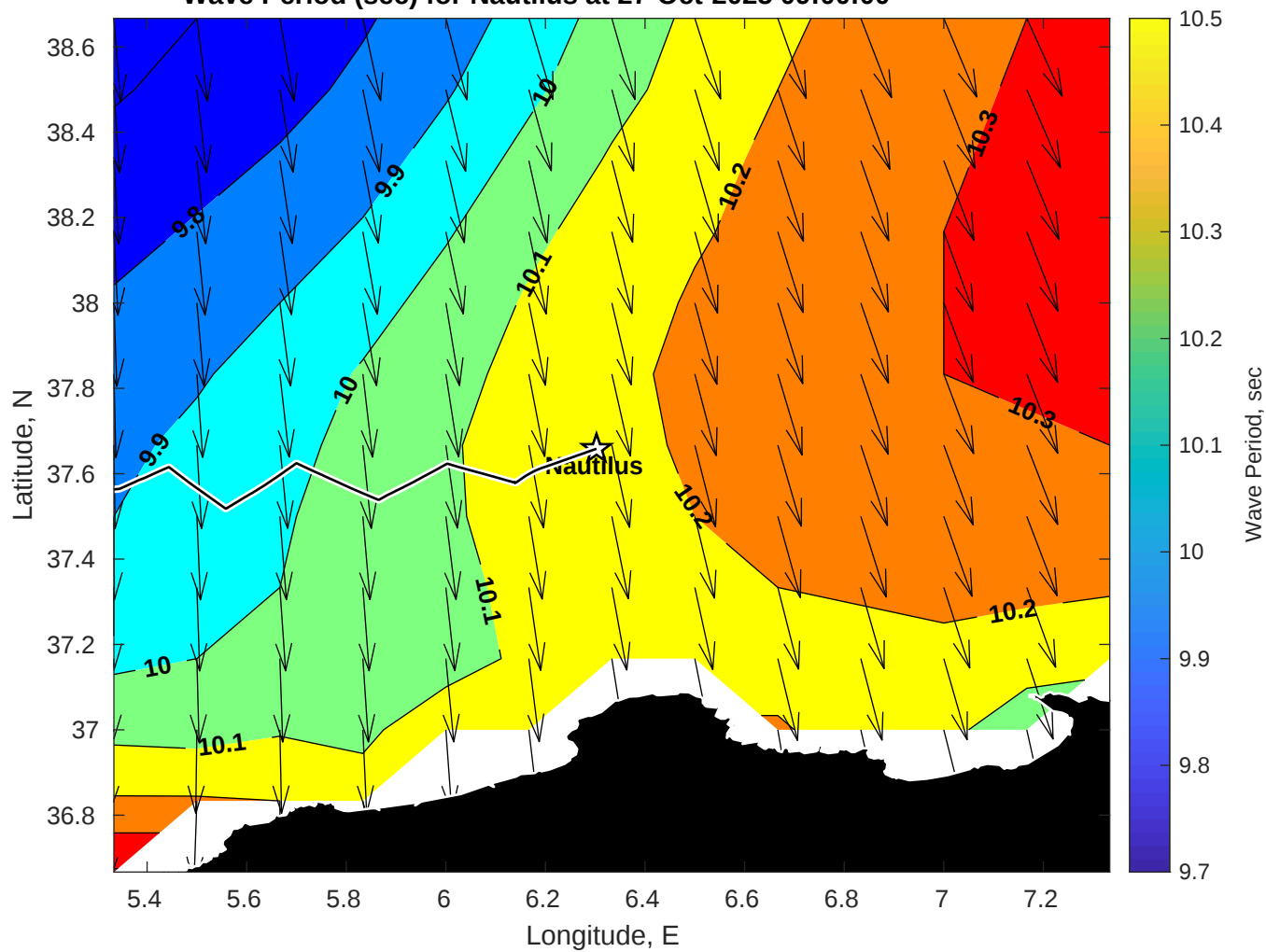
Wave Period (sec) for Nautilus at 27-Oct-2025 09:00:00
