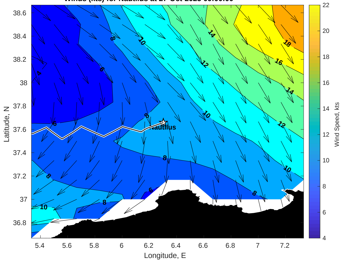
Winds (kts) for Nautilus at 27-Oct-2025 09:00:00
