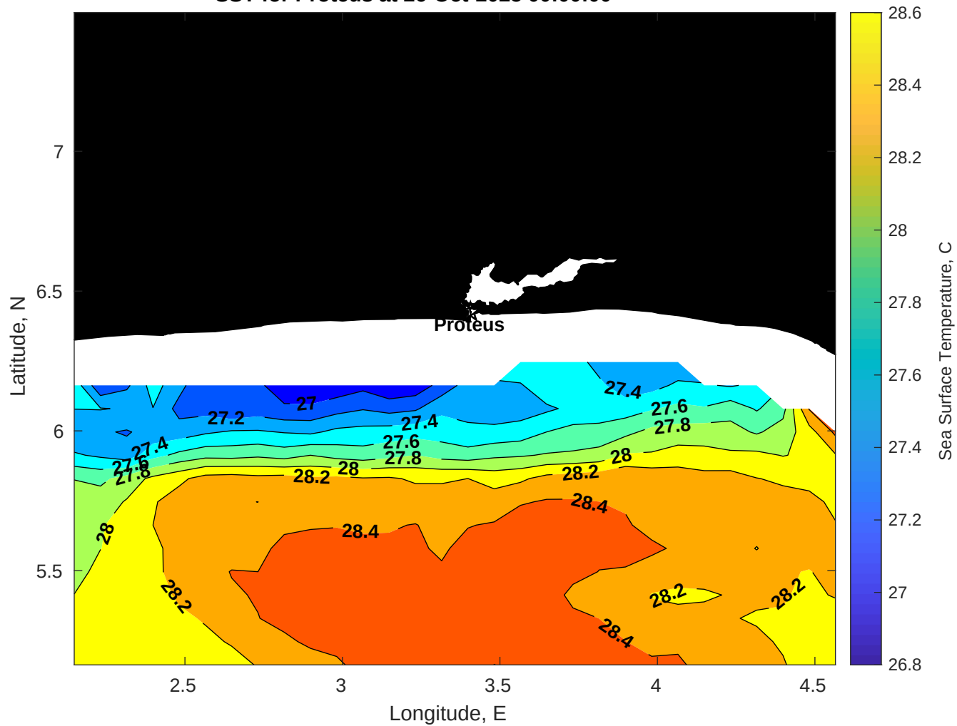
SST for Proteus at 26-Oct-2025 00:00:00
