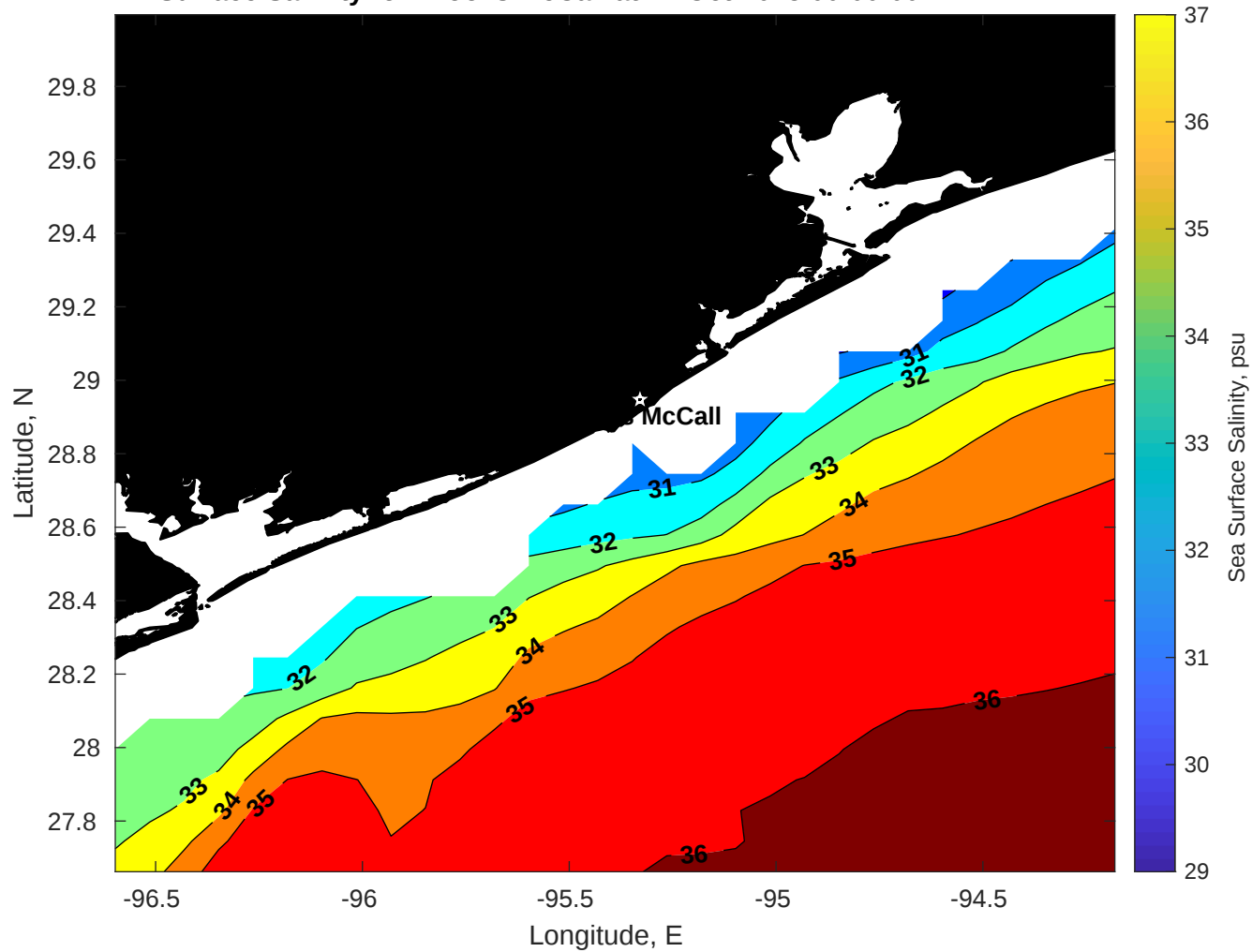
Surface Salinity for Brooks McCall at 27-Oct-2025 00:00:00
