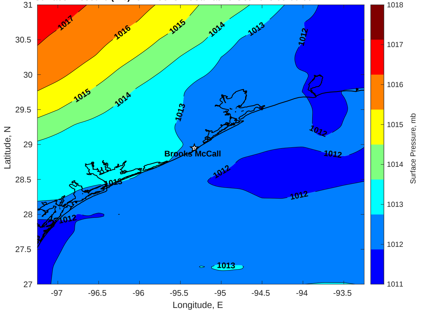
Surface Pressure (mb) for Brooks McCall at 29-Oct-2025 00:00:00
