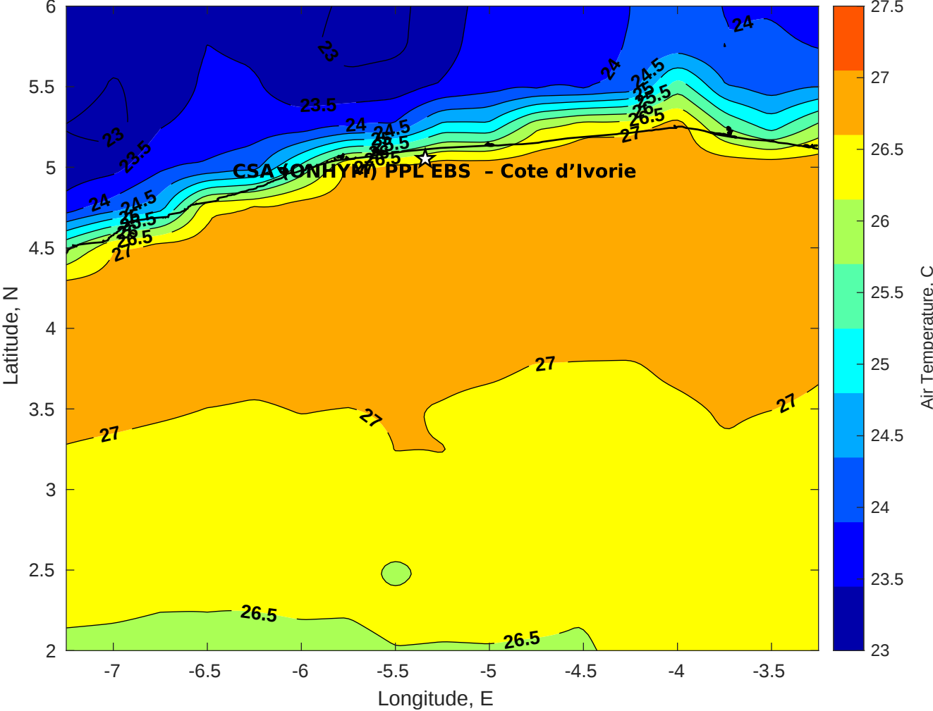
Air Temperature (C) for CSA (ONHYM) PPL EBS - Cote d'Ivoire at 28-Oct-2025
