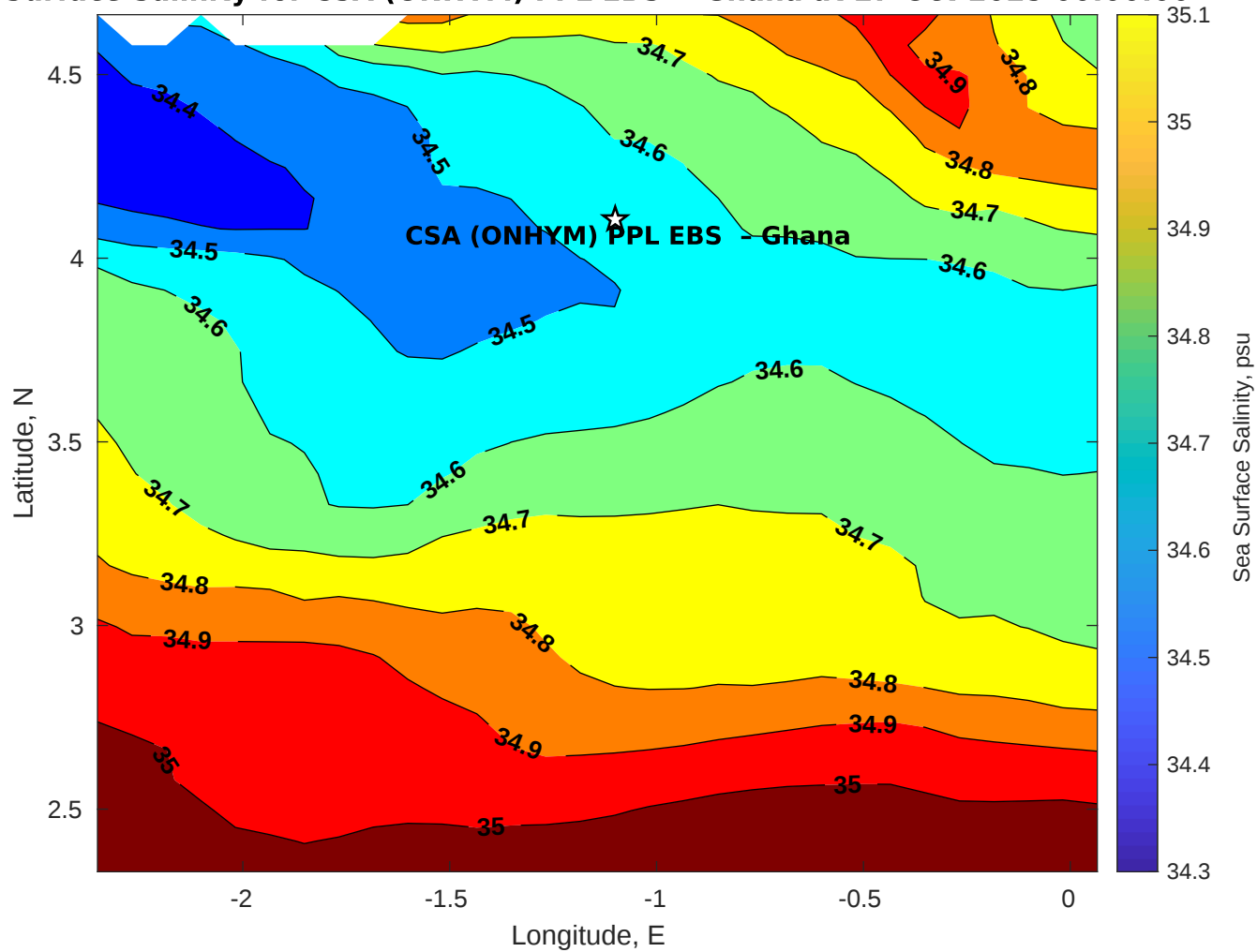
Surface Salinity for CSA (ONHYM) PPL EBS - Ghana at 27-Oct-2025 00:00:00
