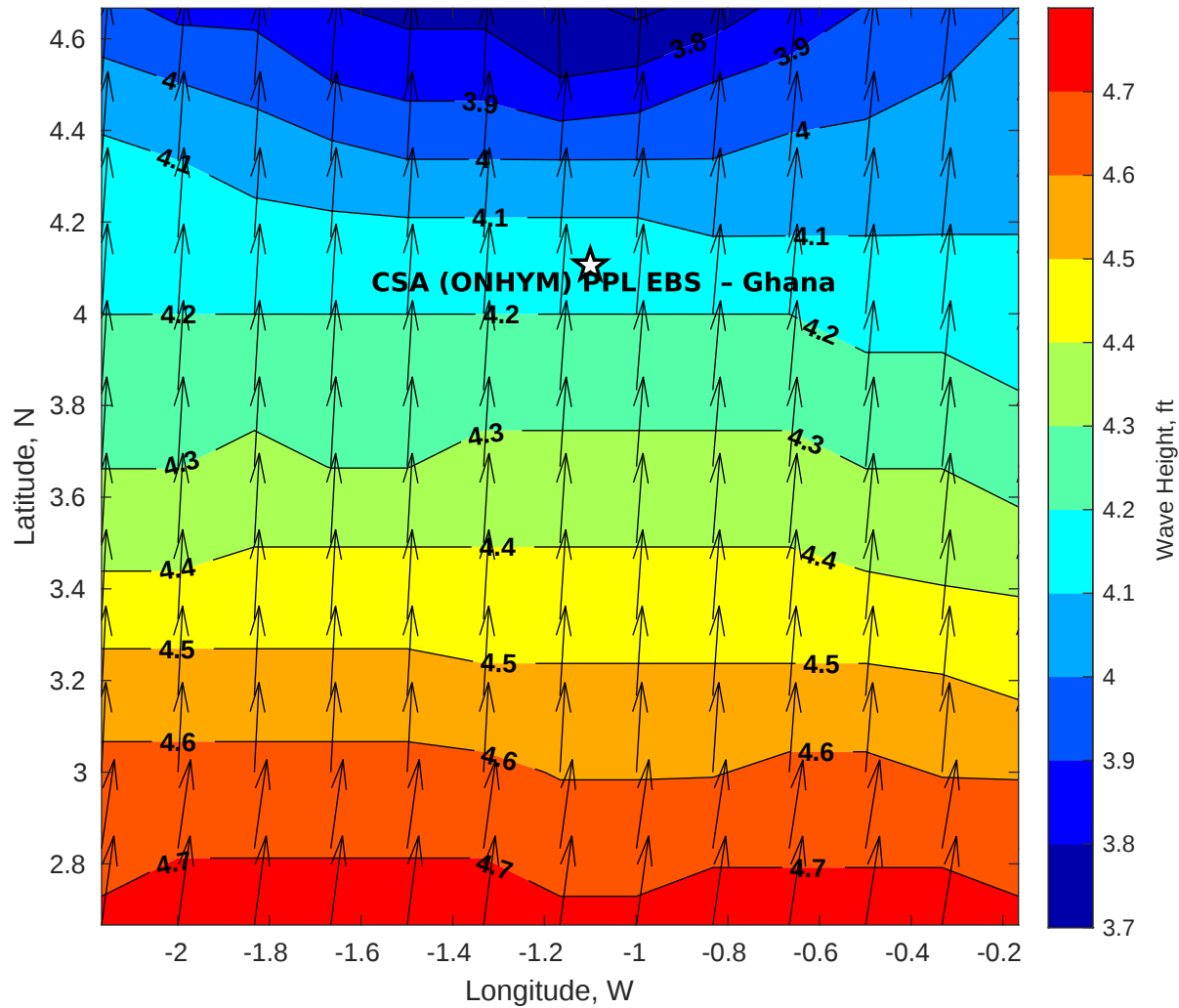
Wave Height (ft) for CSA (ONHYM) PPL EBS - Ghana at 28-Oct-2025 09:00:00
