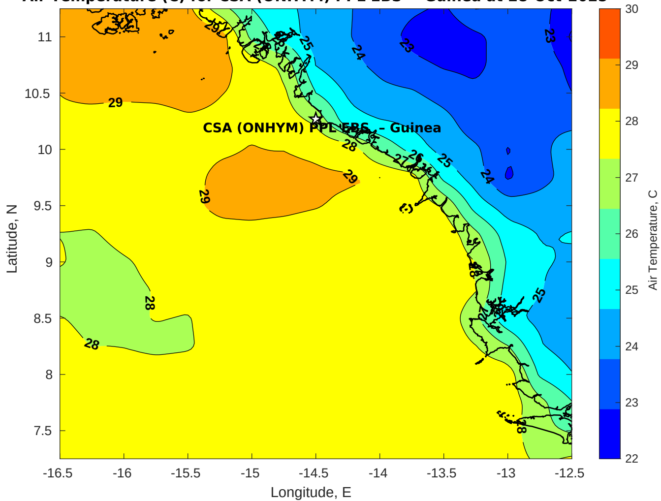
Air Temperature (C) for CSA (ONHYM) PPL EBS - Guinea at 28-Oct-2025
