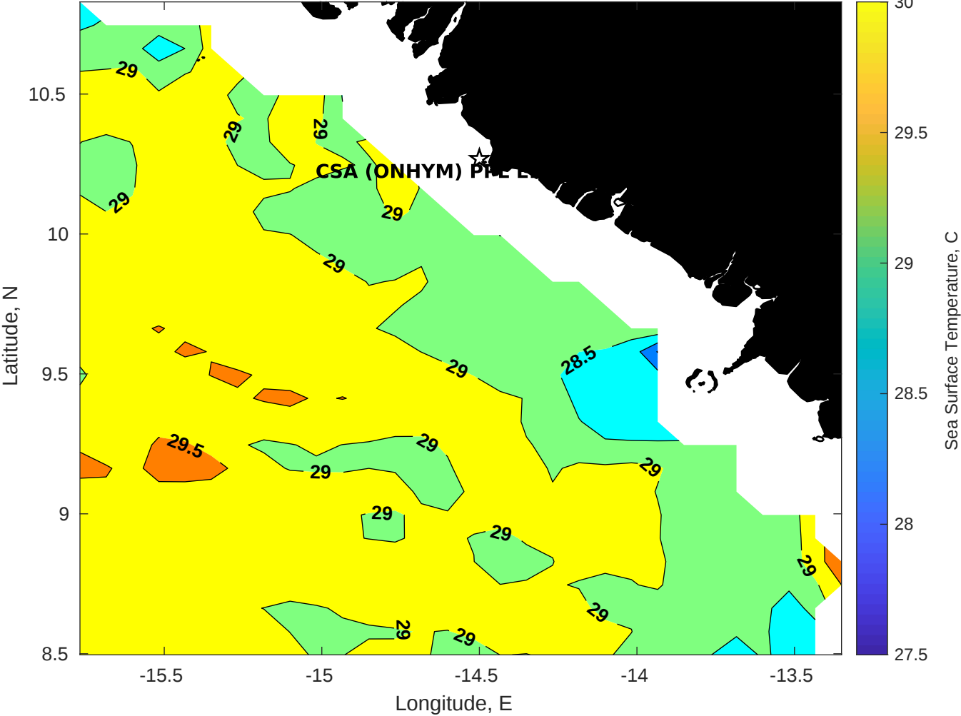
SST for CSA (ONHYM) PPL EBS - Guinea at 27-Oct-2025 00:00:00
