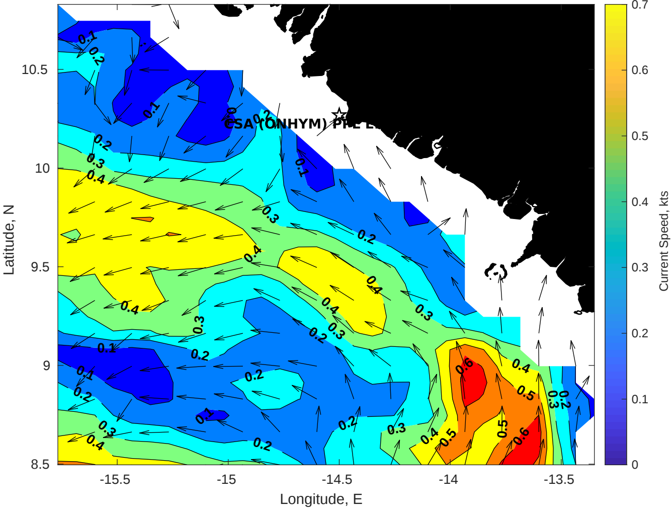
Surface Currents for CSA (ONHYM) PPL EBS - Guinea at 27-Oct-2025 00:00:00
