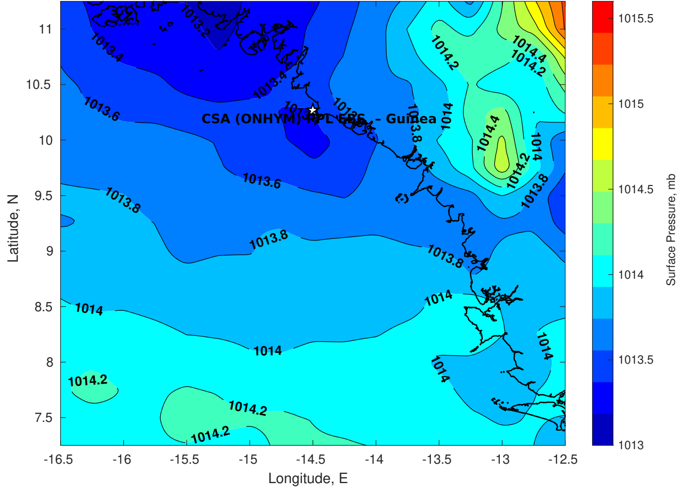
Surface Pressure (mb) for CSA (ONHYM) PPL EBS - Guinea at 30-Oct-2025 00:00:00
