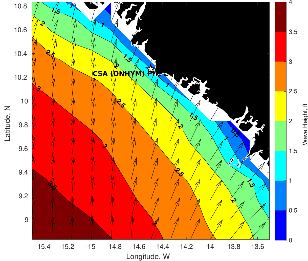
Wave Height (ft) for CSA (ONHYM) PPL EBS - Guinea at 28-Oct-2025 09:00:00
