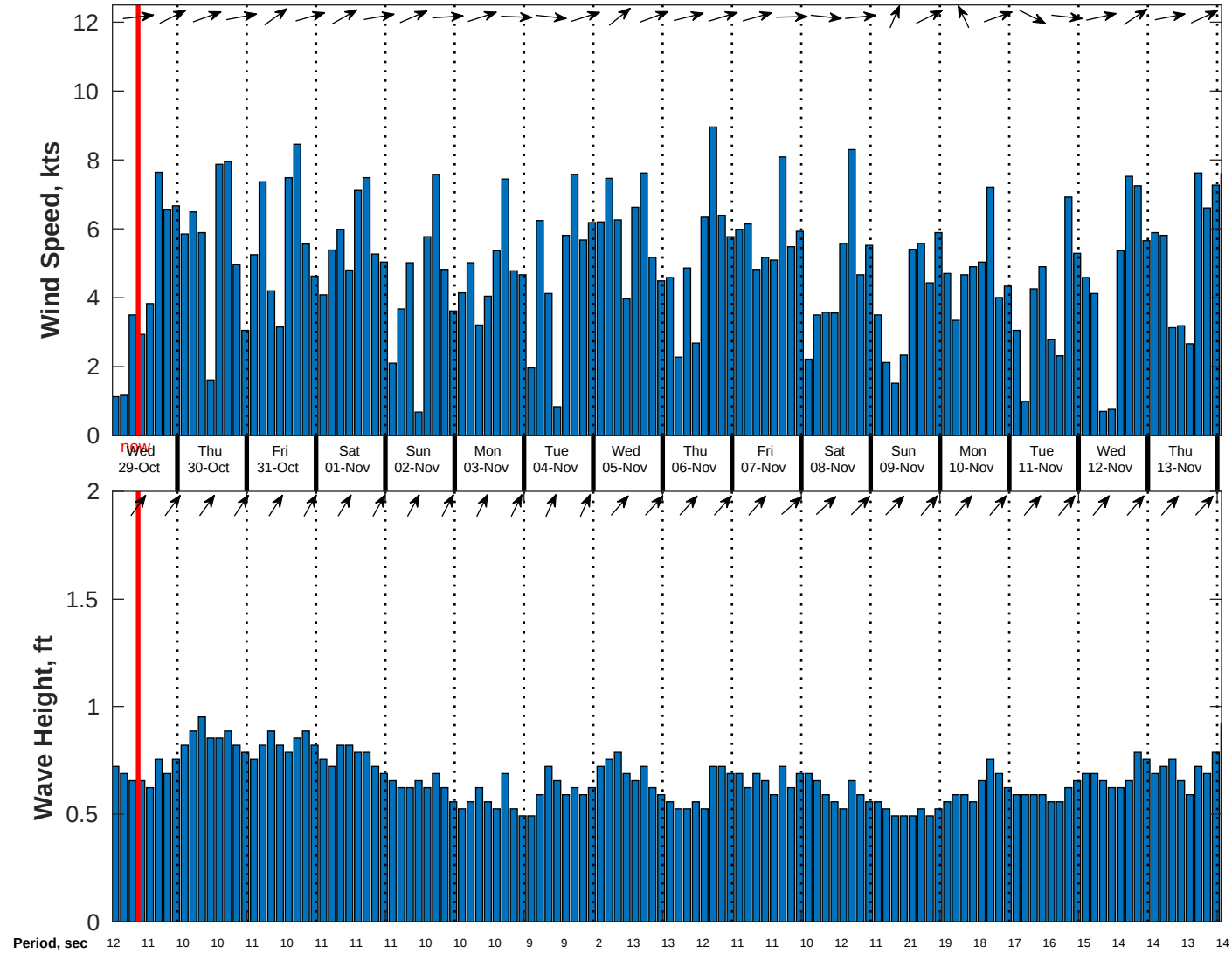
Wind & Wave Forecast for CSA (ONHYM) PPL EBS - Guinea from 28-Oct-2025 01:00:00 to 13-Nov-2025 01:00:00
