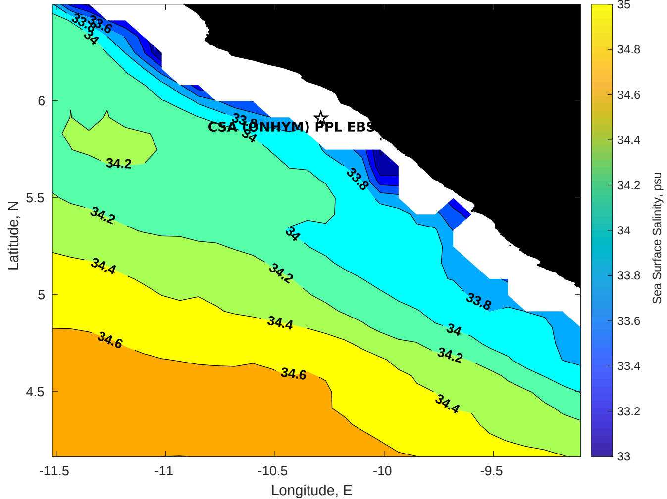
Surface Salinity for CSA (ONHYM) PPL EBS - Liberia at 27-Oct-2025 00:00:00
