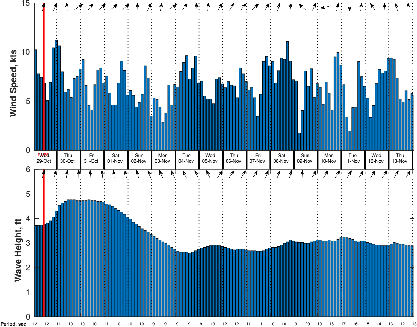
Wind & Wave Forecast for CSA (ONHYM) PPL EBS - Liberia from 28-Oct-2025 01:00:00 to 13-Nov-2025 01:00:00
