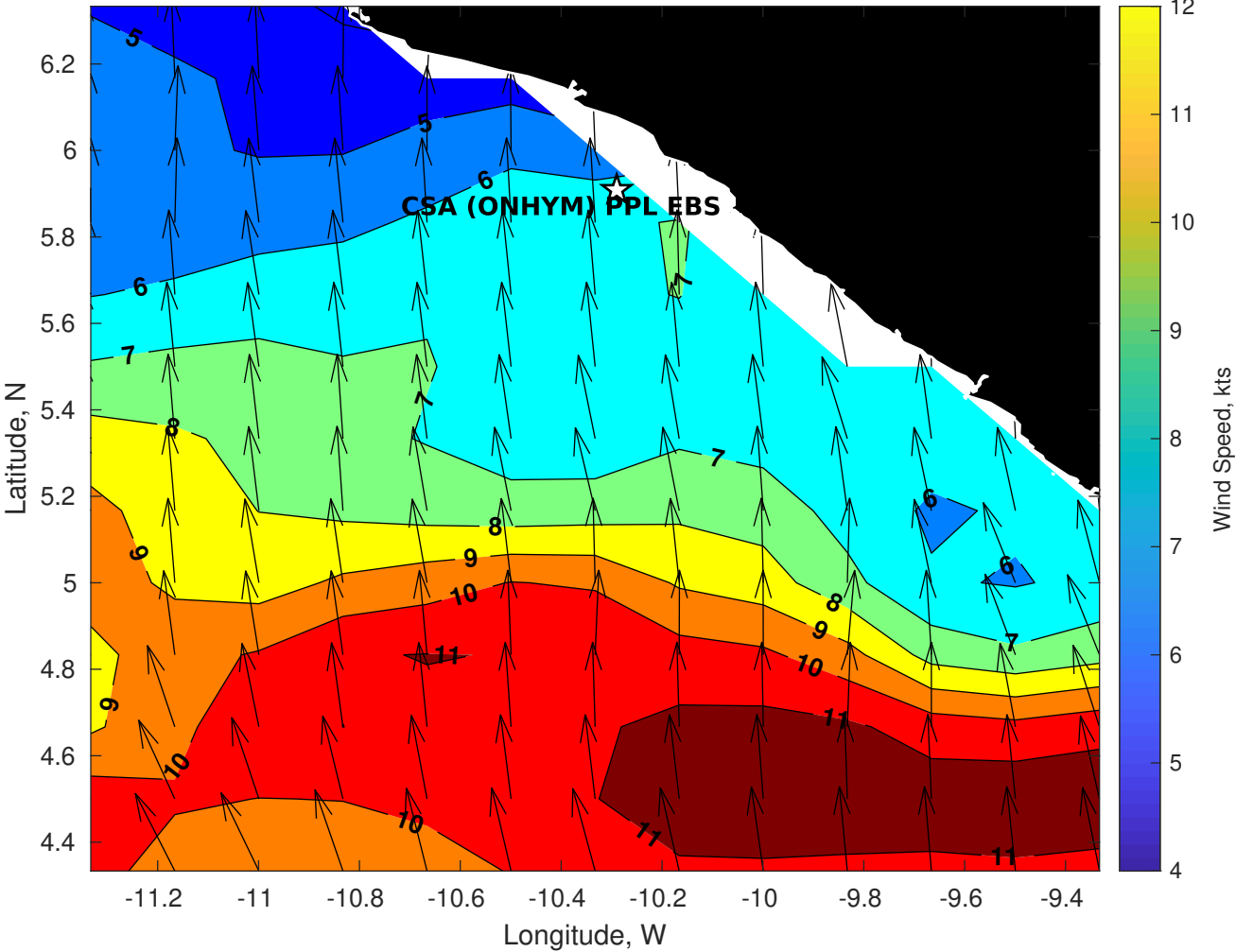
Winds (kts) for CSA (ONHYM) PPL EBS - Liberia at 28-Oct-2025 09:00:00
