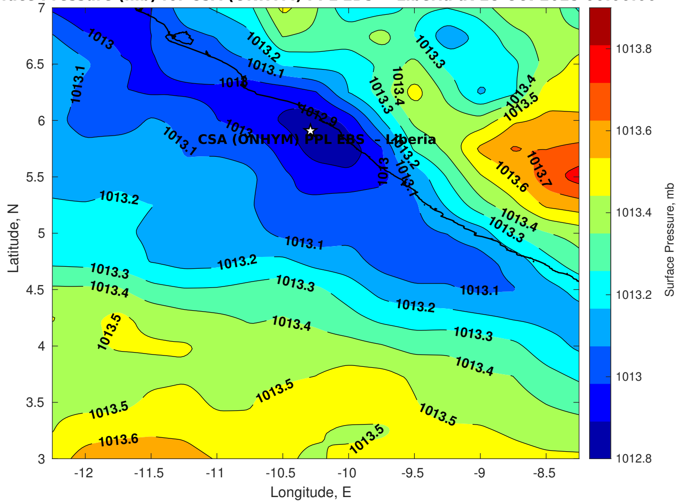
Surface Pressure (mb) for CSA (ONHYM) PPL EBS - Liberia at 28-Oct-2025 00:00:00
