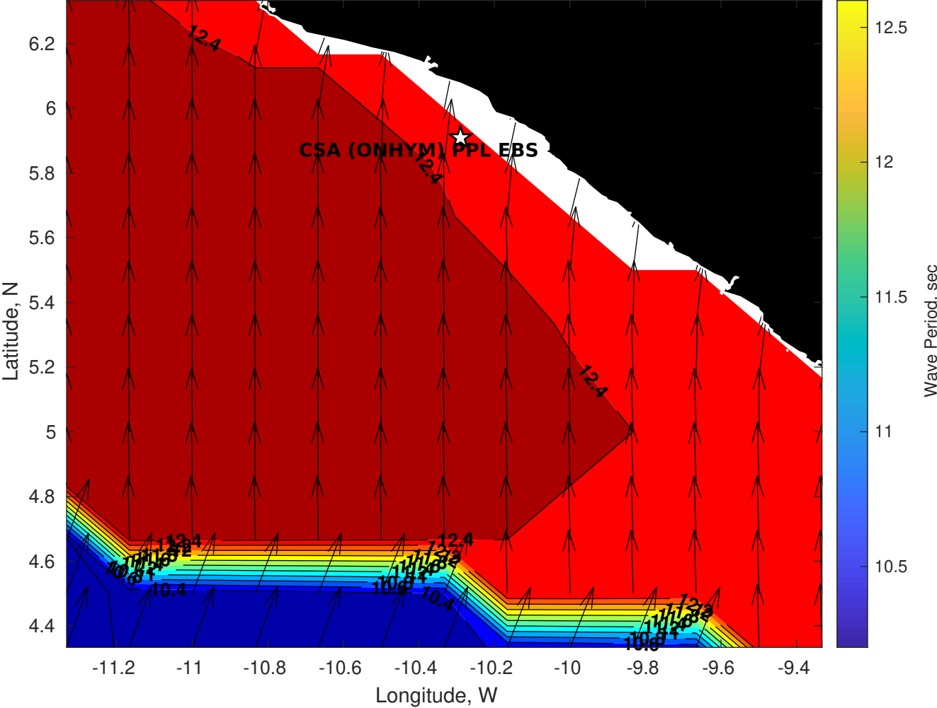
Wave Period (sec) for CSA (ONHYM) PPL EBS - Liberia at 28-Oct-2025 09:00:00
