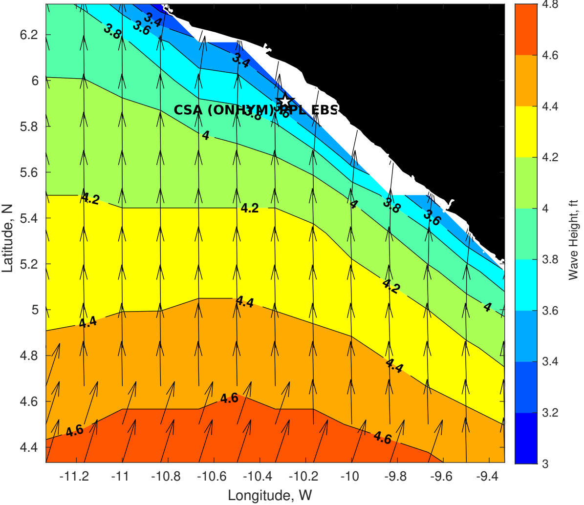
Wave Height (ft) for CSA (ONHYM) PPL EBS - Liberia at 28-Oct-2025 09:00:00
