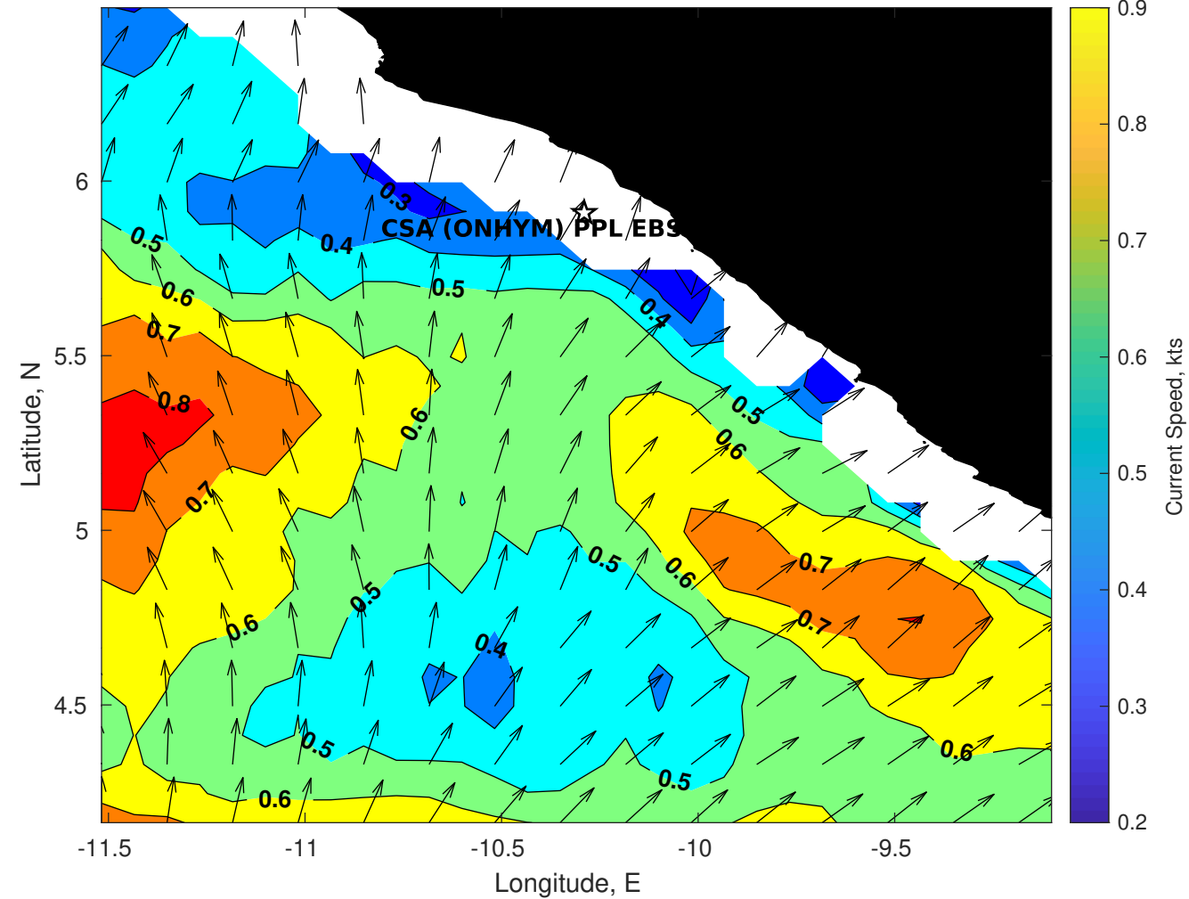
Surface Currents for CSA (ONHYM) PPL EBS - Liberia at 27-Oct-2025 00:00:00
