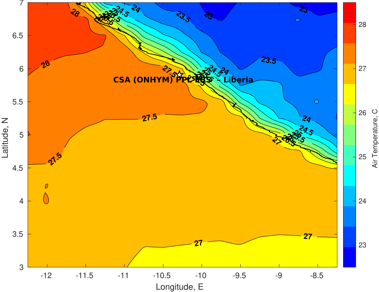
Air Temperature (C) for CSA (ONHYM) PPL EBS - Liberia at 28-Oct-2025
