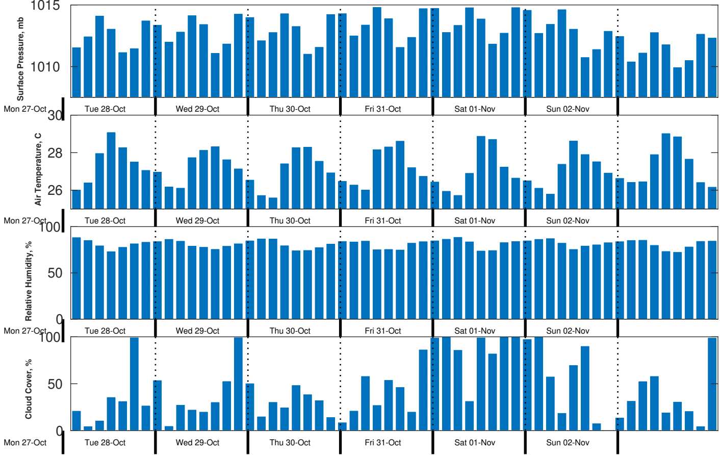
Met Forecast for CSA (ONHYM) PPL EBS - Liberia from 28-Oct-2025 00:00:00 to 04-Nov-2025 00:00:00
