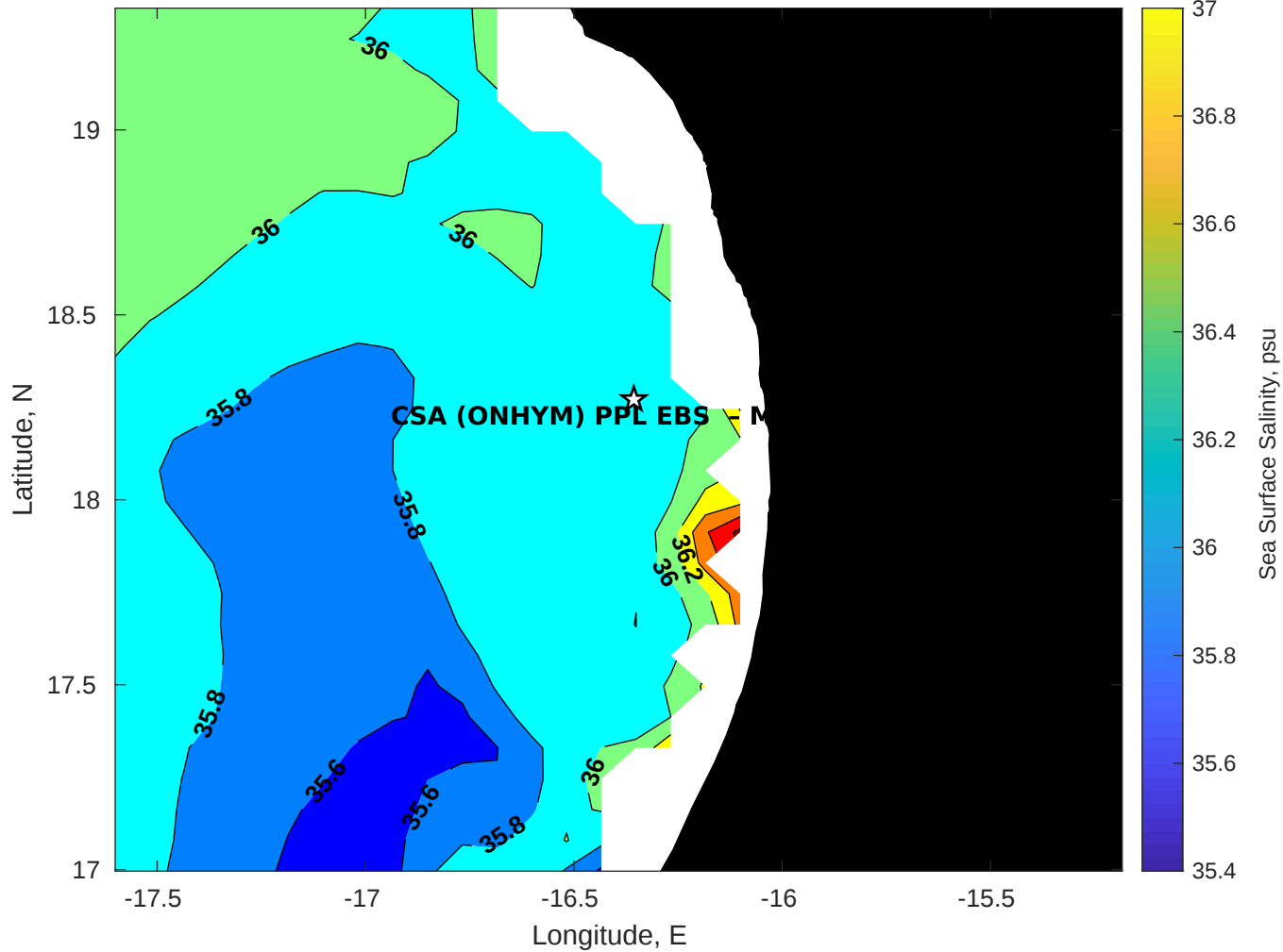
Surface Salinity for CSA (ONHYM) PPL EBS - Mauritania at 27-Oct-2025 00:00:00
