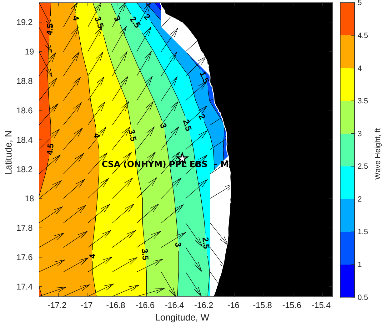
Wave Height (ft) for CSA (ONHYM) PPL EBS - Mauritania at 28-Oct-2025 09:00:00
