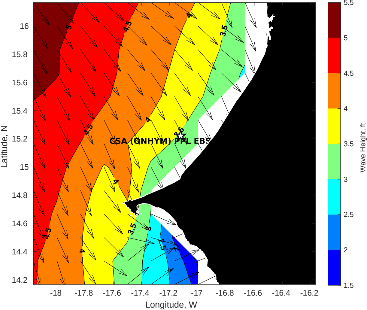
Wave Height (ft) for CSA (ONHYM) PPL EBS - Senegal at 28-Oct-2025 09:00:00
