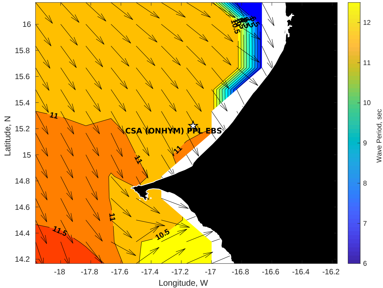
Wave Period (sec) for CSA (ONHYM) PPL EBS - Senegal at 28-Oct-2025 09:00:00
