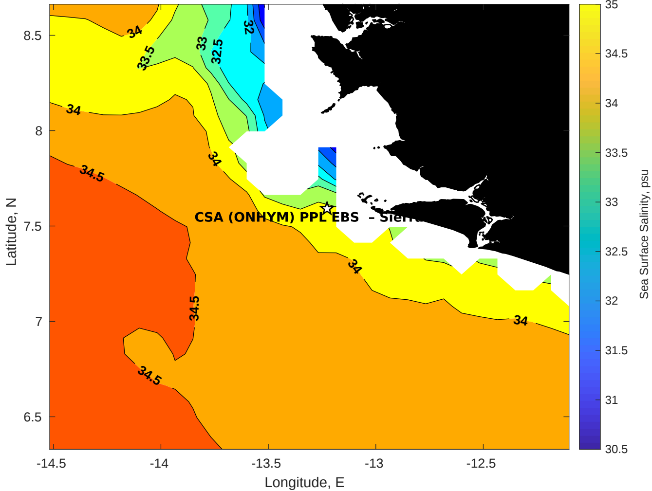
Surface Salinity for CSA (ONHYM) PPL EBS - Sierra Leone at 27-Oct-2025 00:00:00
