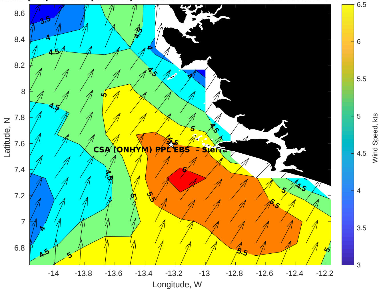
Winds (kts) for CSA (ONHYM) PPL EBS - Sierra Leone at 28-Oct-2025 09:00:00
