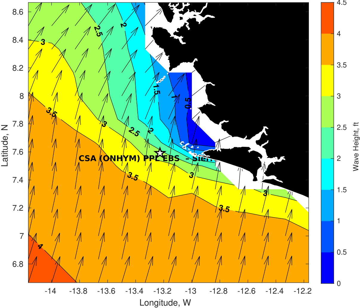
Wave Height (ft) for CSA (ONHYM) PPL EBS - Sierra Leone at 28-Oct-2025 09:00:00
