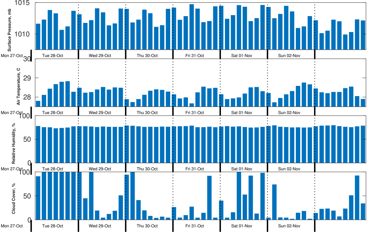
Met Forecast for CSA (ONHYM) PPL EBS - Sierra Leone from 28-Oct-2025 00:00:00 to 04-Nov-2025 00:00:00
